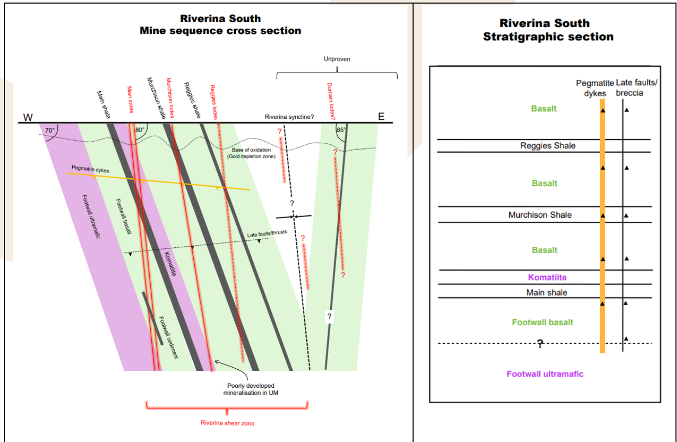
Figure 2 – Diagrammatic cross section of the defined mine sequence of the Riverina Deposit and indicative stratigraphic section.
