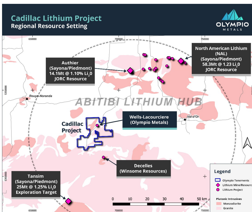
Figure 5: Location of Cadillac Project relative to intrusive bodies and lithium mineralisation
