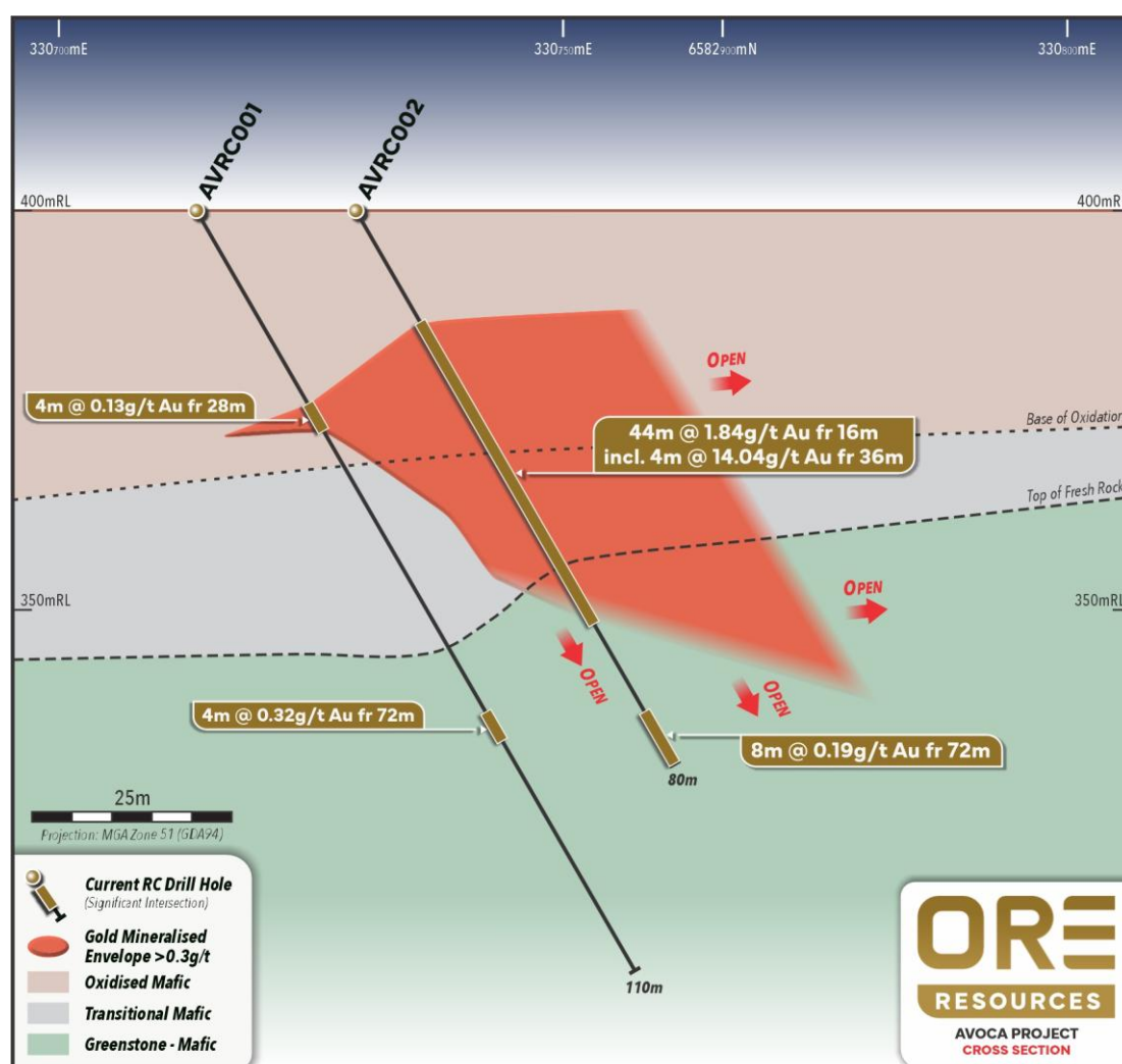
Figure 3: Cross Section – AVRC002
