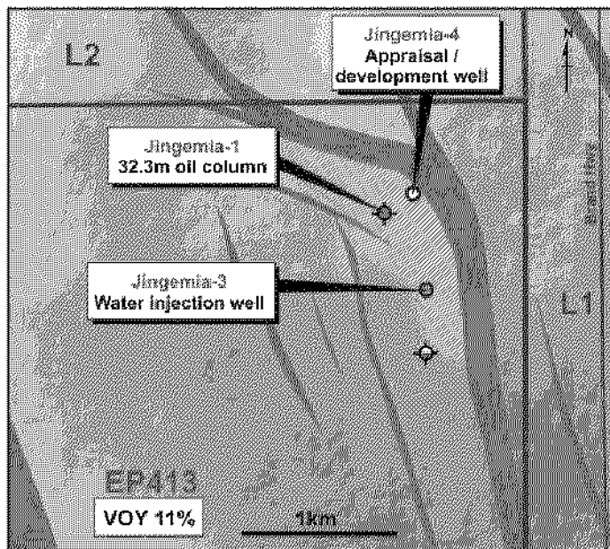
Schematic structure map of the Jingemia oil field.
