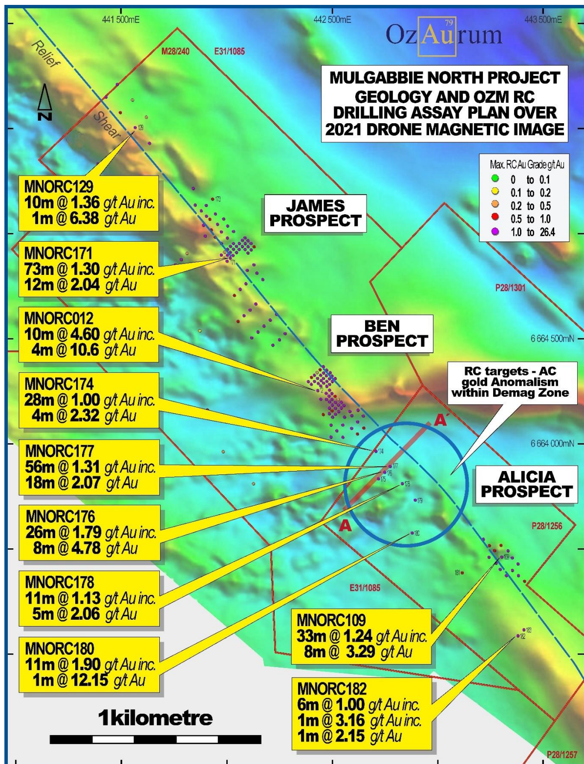
Figure 2: Mulgabbie North 1VD magnetic image with current drill results and previously released RC results.
