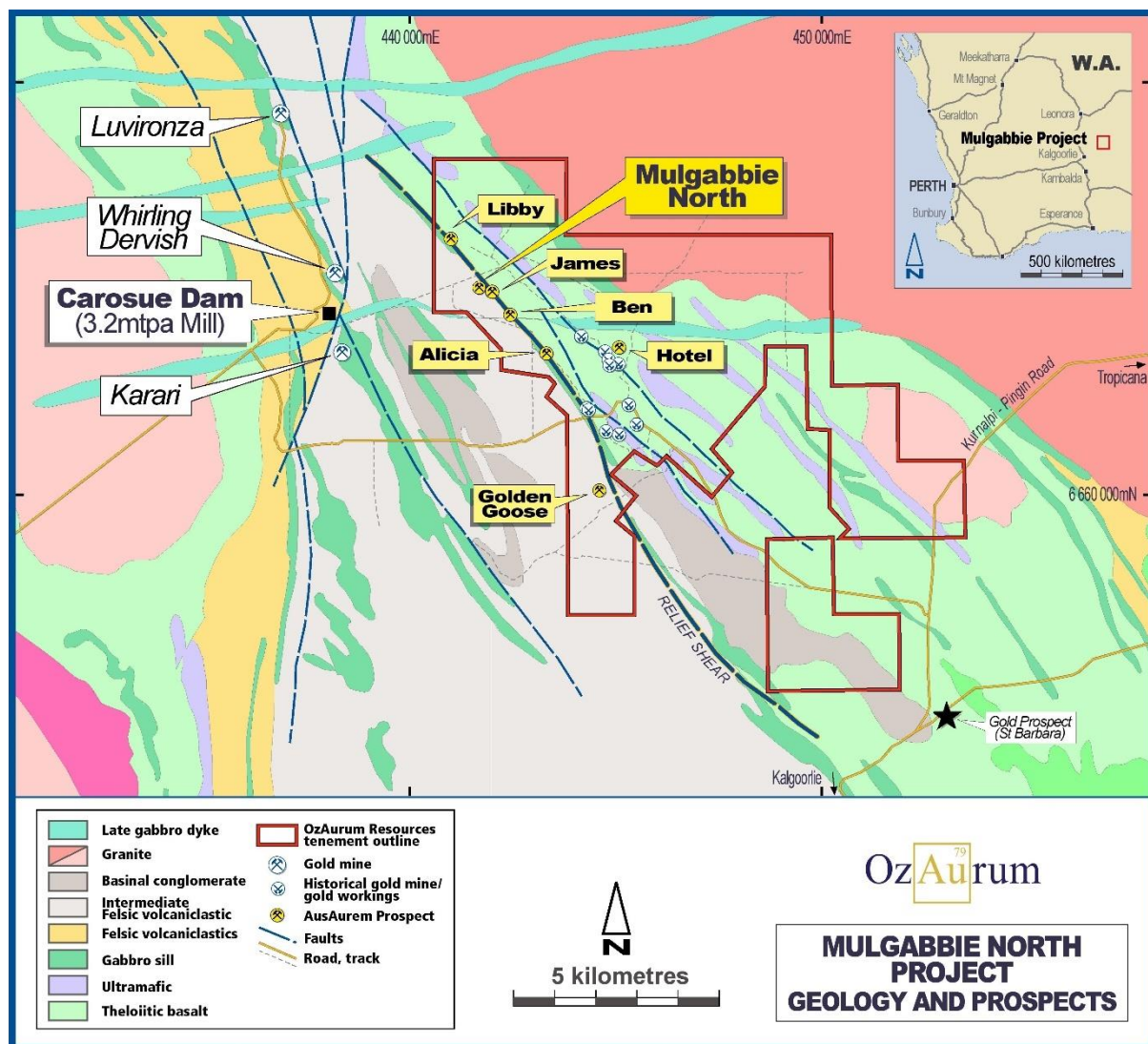
Figure 4: Mulgabbie North Project
