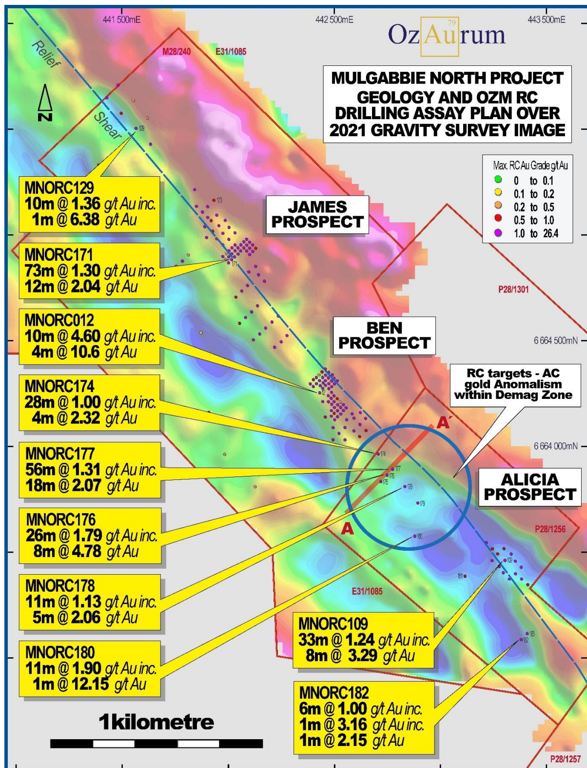
Figure 3: Mulgabbie North gravity image with current drill results and previously released RC drill results.
