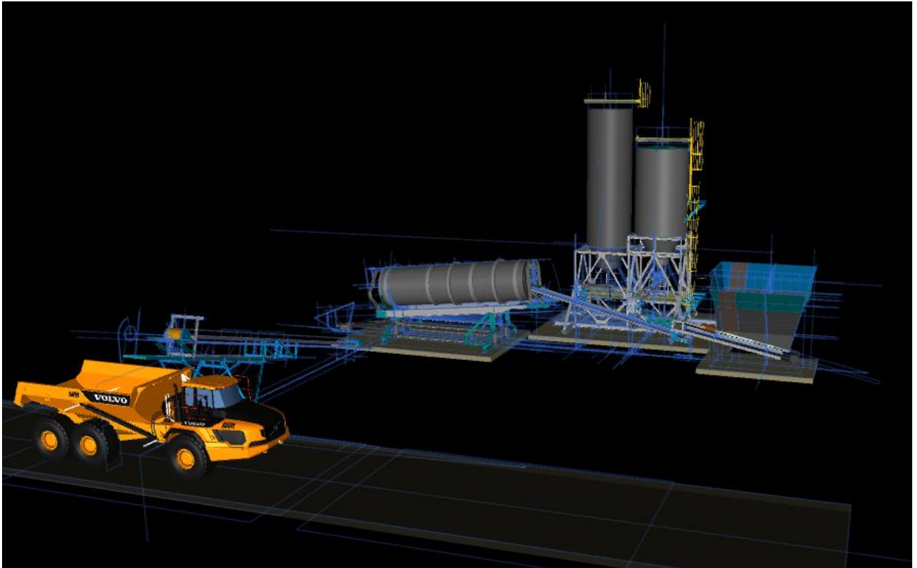
Figure 5: The 3D CAD model of the heap leach plant
