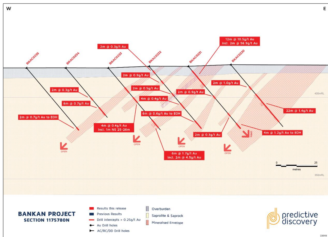
Figure 4 - 800W Prospect, Section 1175780N with six new AC holes BKAC0230 to BKAC0235.
