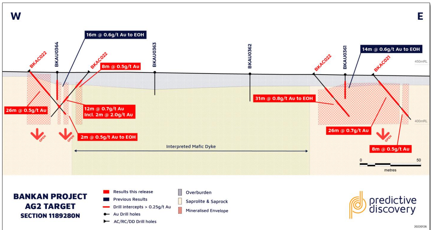
Figure 7 – Section 1189280N with new aircore holes BKAC0219, BKAC0220, BKAC0221 and BKAC0224 showing interpreted Mafic Dyke.
