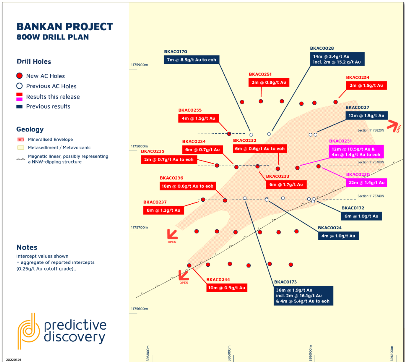
Figure 2 - 800W Prospect, showing new gold intercepts overlain on earlier drill results.
