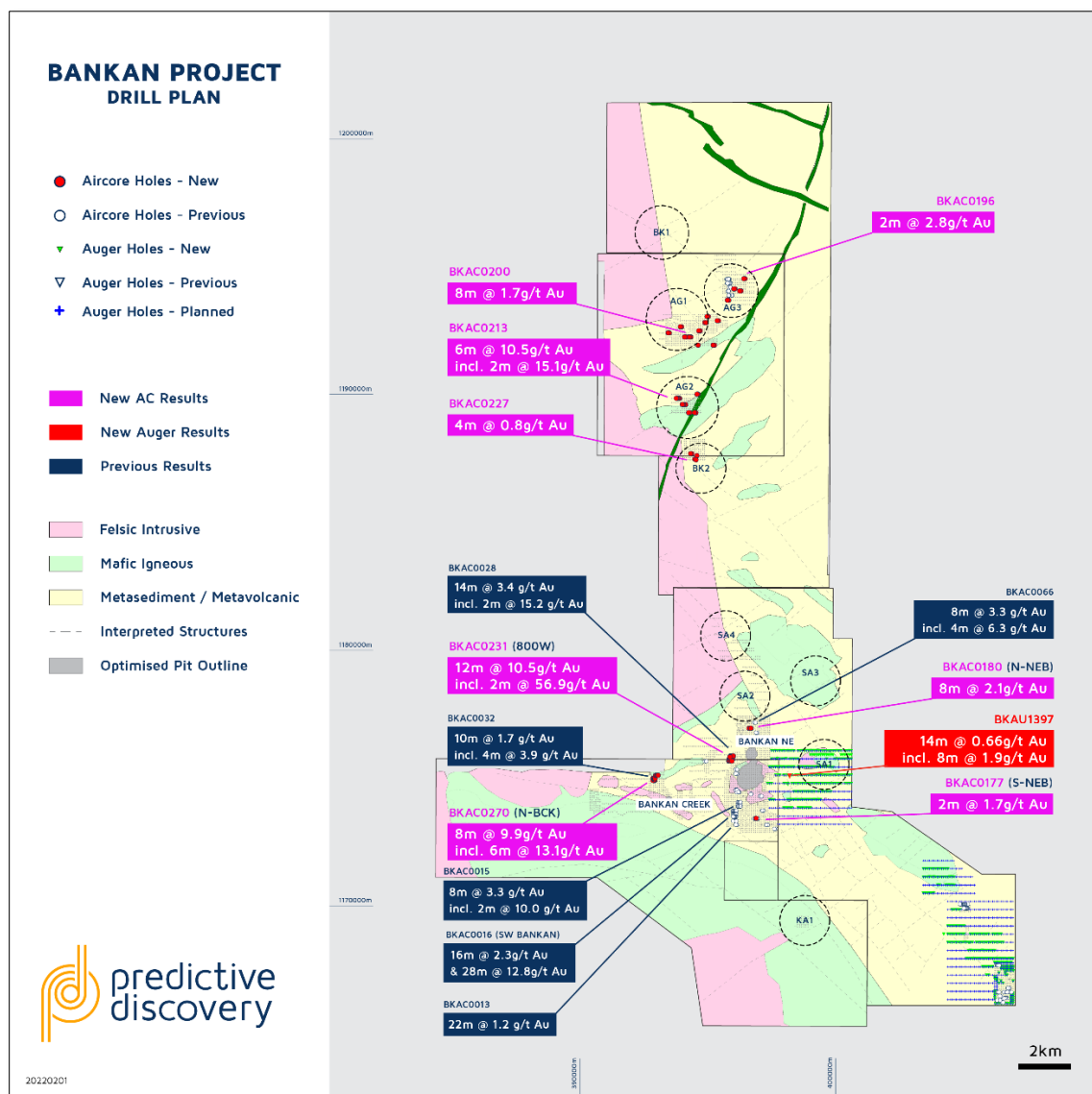
Figure 1 – Bankan Project, new regional AC/Auger results overlain on previous regional results and interpreted geology.
