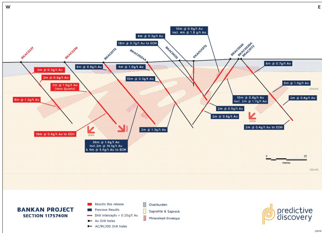
Figure 3 - 800W Prospect, Section 1175740N with new AC holes BKAC0236 and BKAC0237 overlain on previous AC and power auger drilling.
