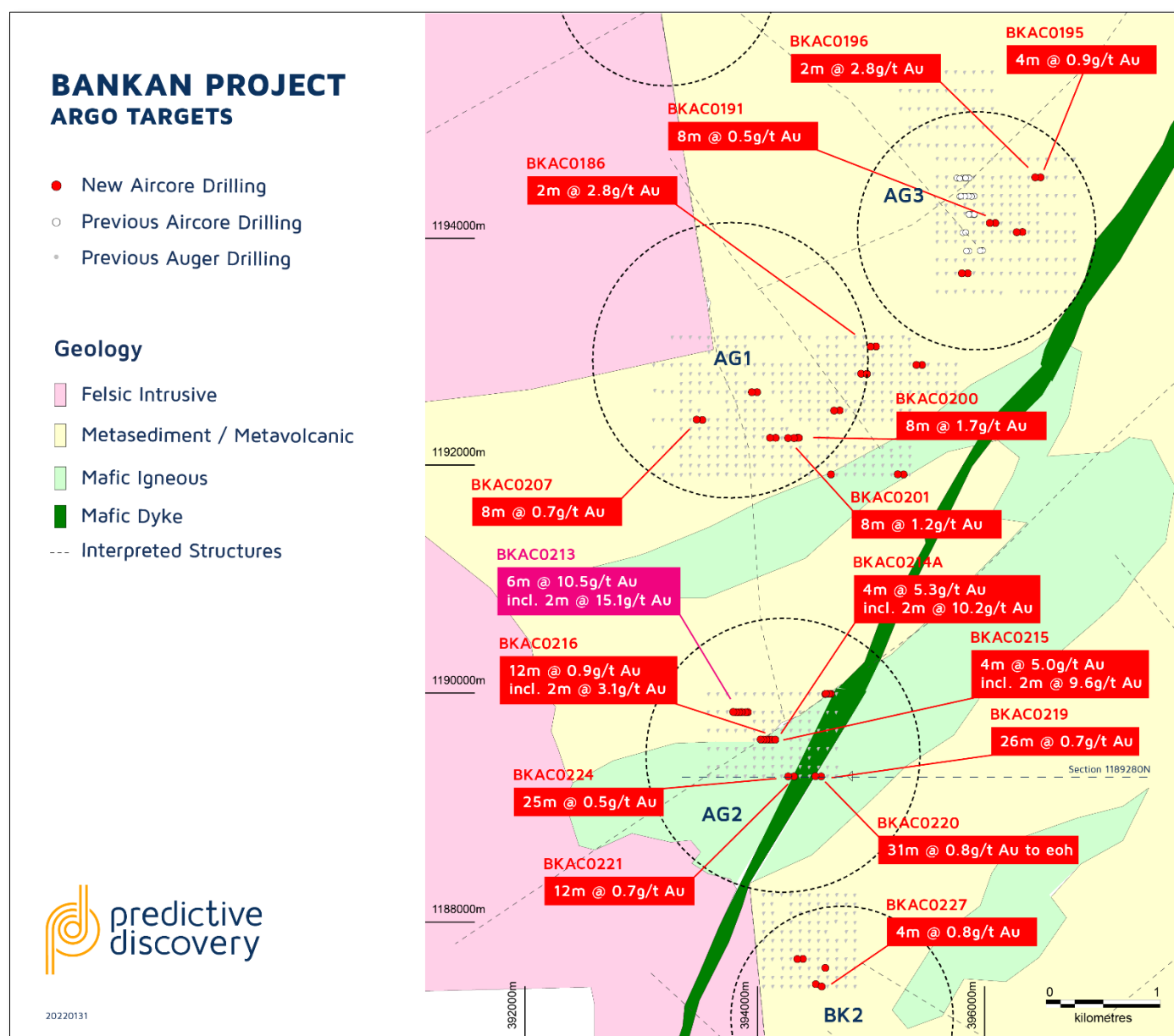
Figure 6 – Argo Exploration Permit (Part of the Bankan Project) with Aircore holes BKAC0181 - BKAC0229 and new results overlain on previously completed auger grids.
