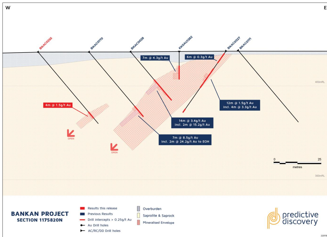
Figure 5 - 800W Prospect, Section 1175780N with new AC hole BKAC0255.
