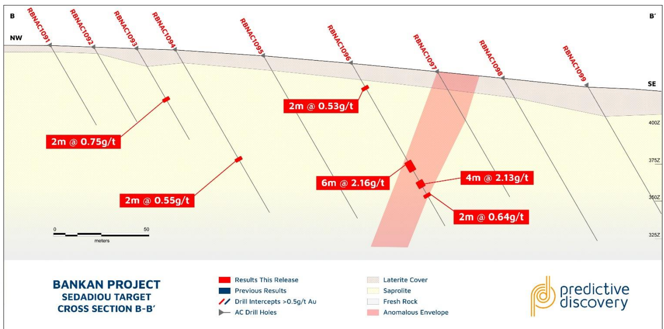
Figure 18: Sedadiou cross section B-B'
