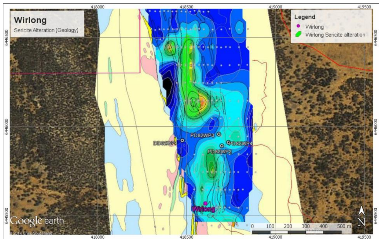
Figure 3: Wirlong sericite alteration and Pb anomaly
