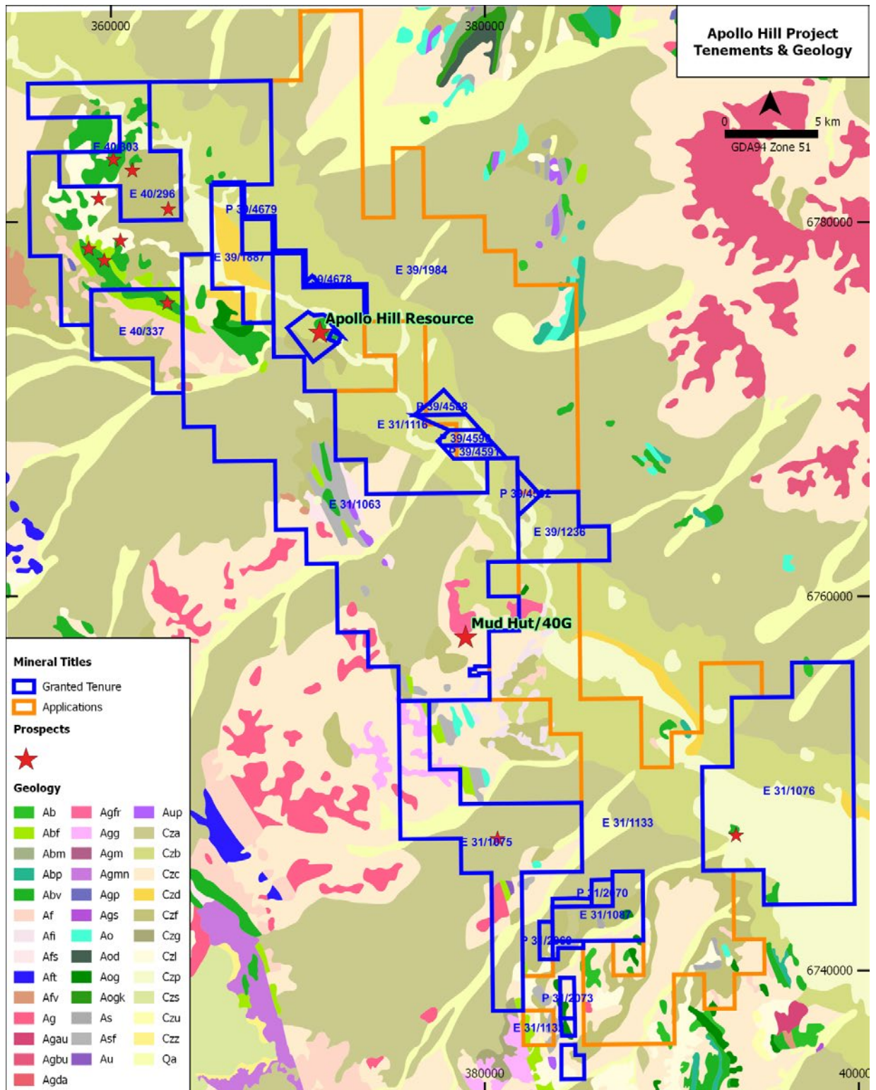
Figure 4 - Apollo Hill Project Tenements & Geology
