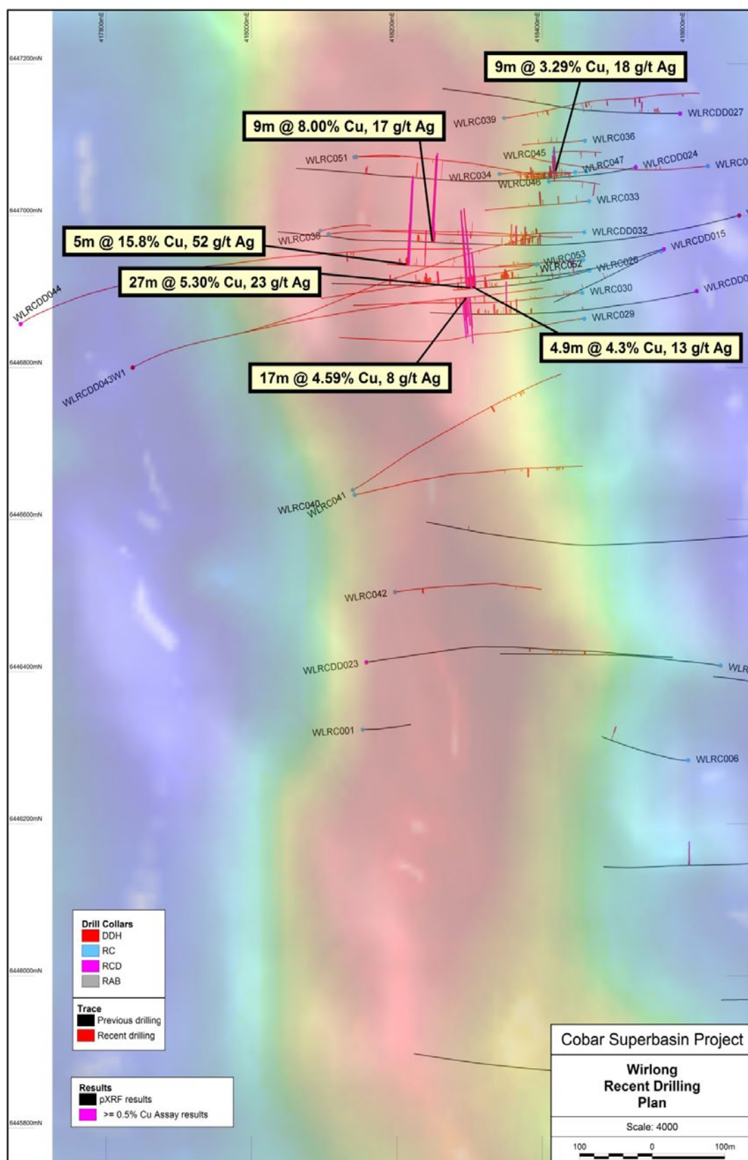
FIGURE 3: WIRLONG PROSPECT MAIN ZONE PLAN VIEW
