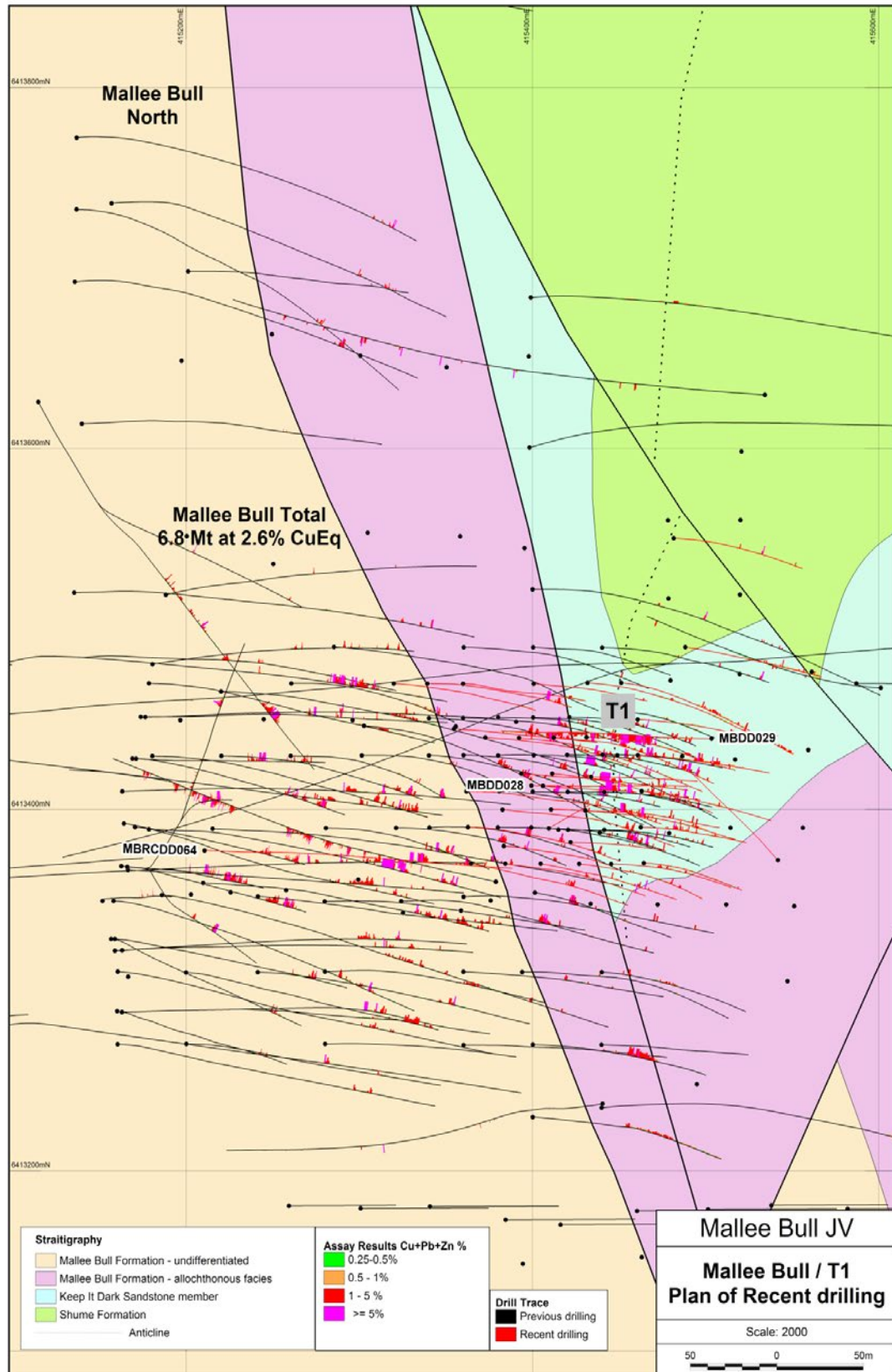
Figure 1: Mallee Bull Drill Plan
