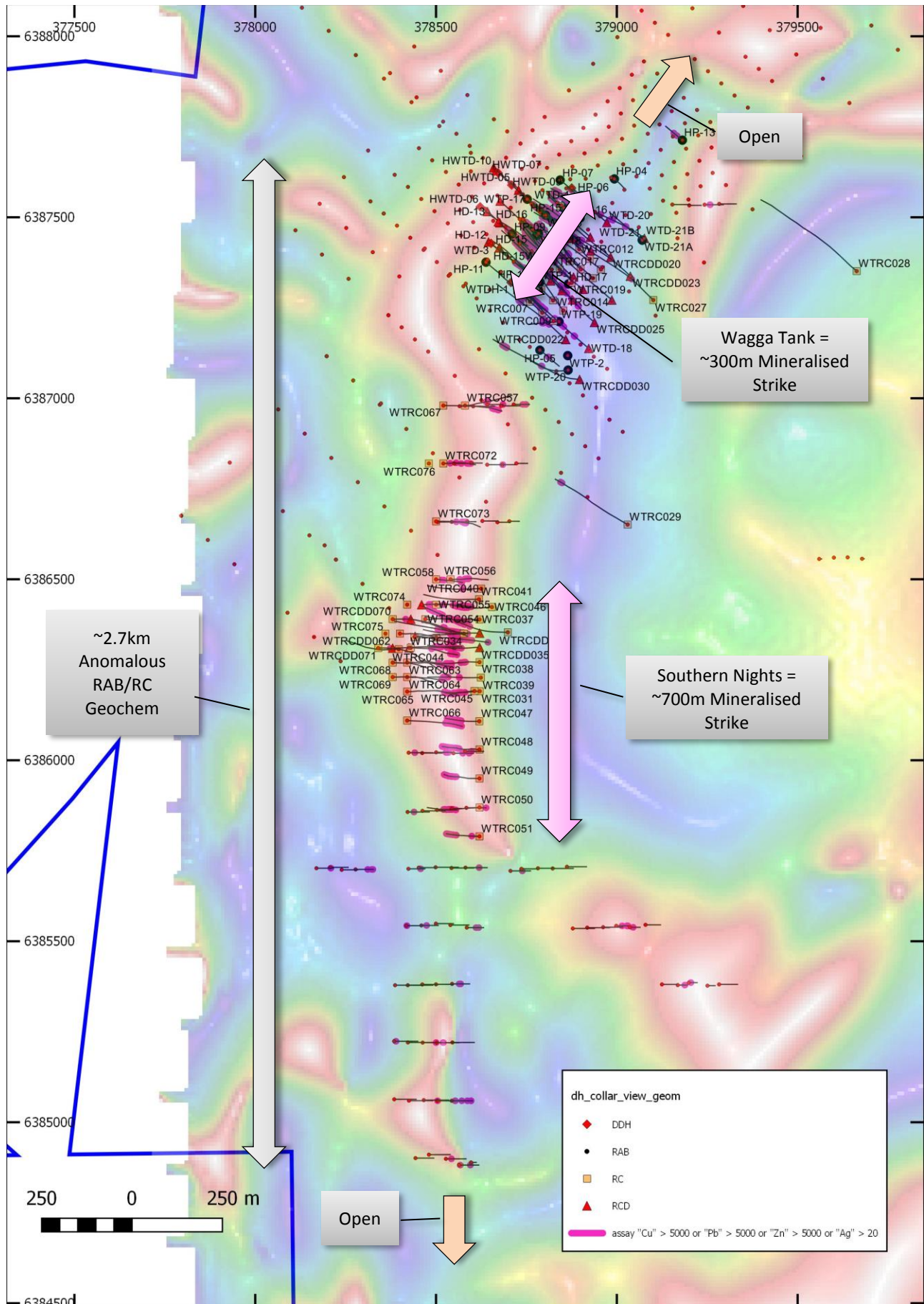
Figure 1 – Wagga Tank/Southern Nights Plan (Zn/Pb Histogram/1VD Magnetics)
