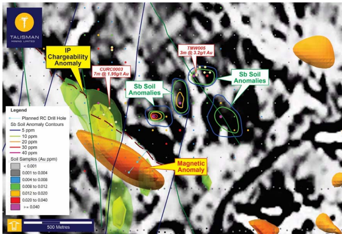
Figure 2: Cumbine Gold Prospect showing previous drilling, IP and magnetic anomalies and proposed RC drilling.
