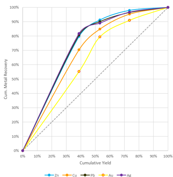
Figure 5. Sample 2 (+31.5mm) Cumulative Yield/Cumulative Metal Recovery Curve
