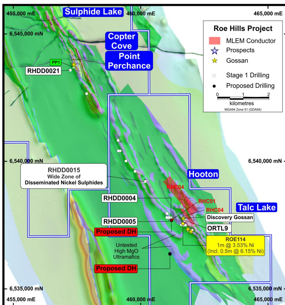
Figure 4. Talc Lake priority drill targets and key geological, geophysical and geochemical references
