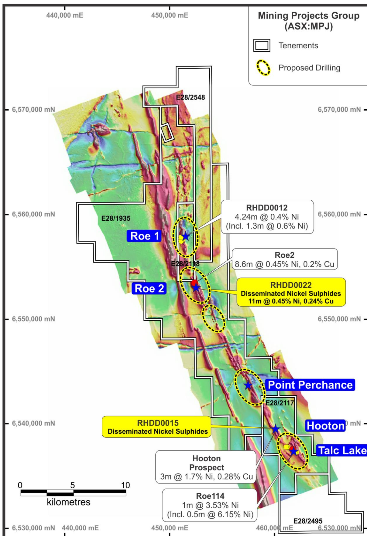
Figure 3. Roe Hills 40km strike with main prospects and proposed priority drilling target areas
