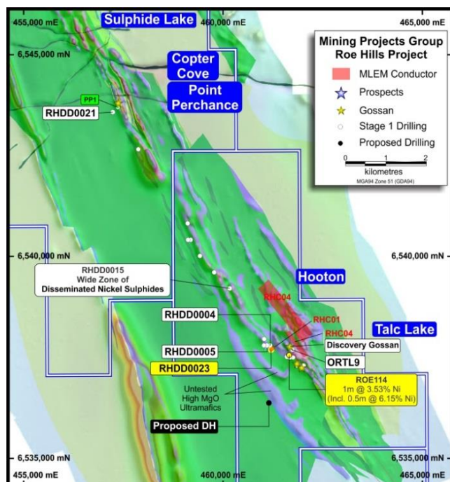
Figure 3. Diamond Hole RHDD0023 Location
