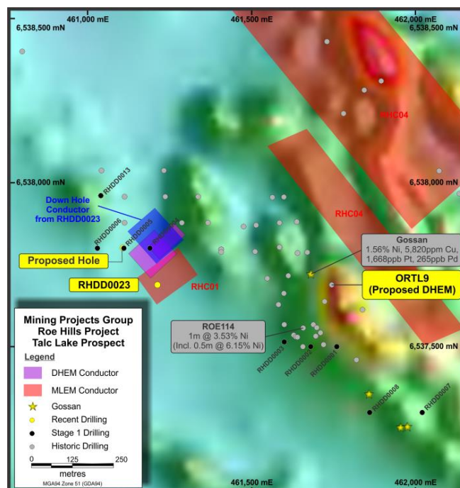
Figure 4. Talc Lake Recent Drilling Conductors
