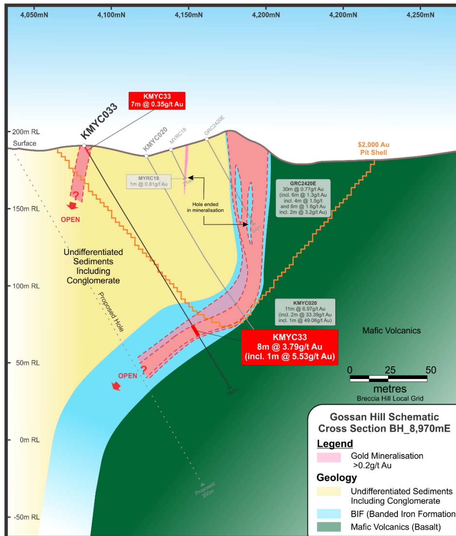
Figure 3. Gossan Hill Schematic Cross-Section, showing the interpreted flattening of the mineralisation as highlighted by hole KMYC033.
