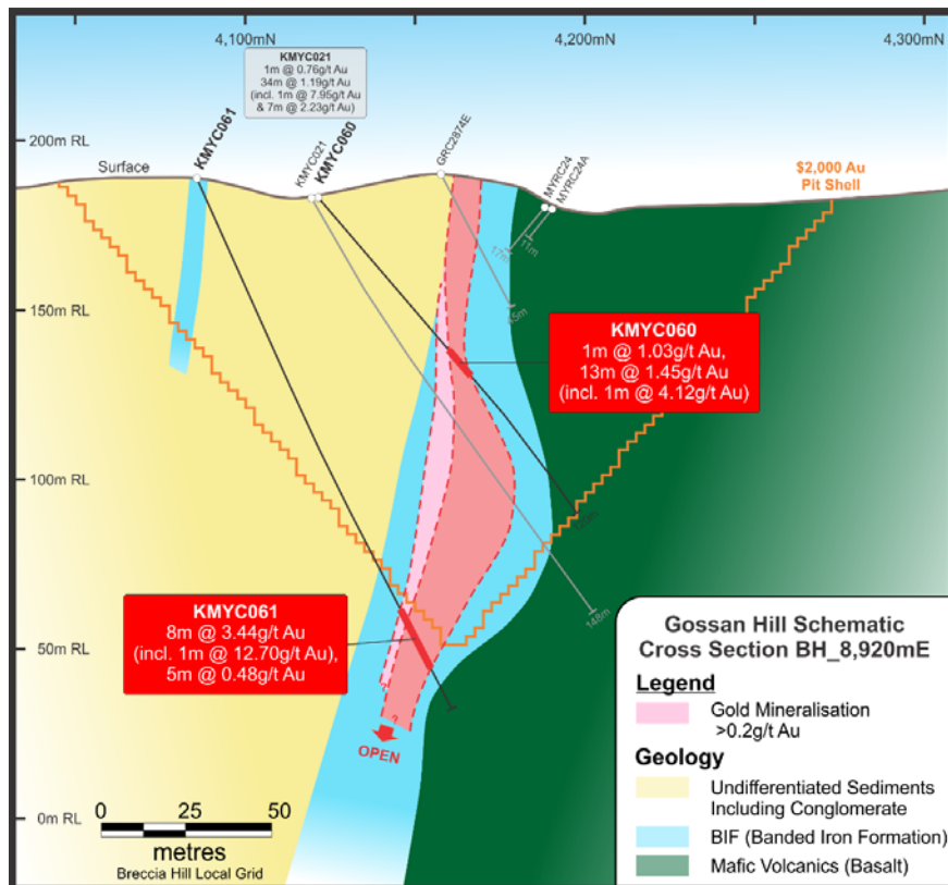
Figure 4. Gossan Hill Schematic Cross-Section, BH_8,920mE.
