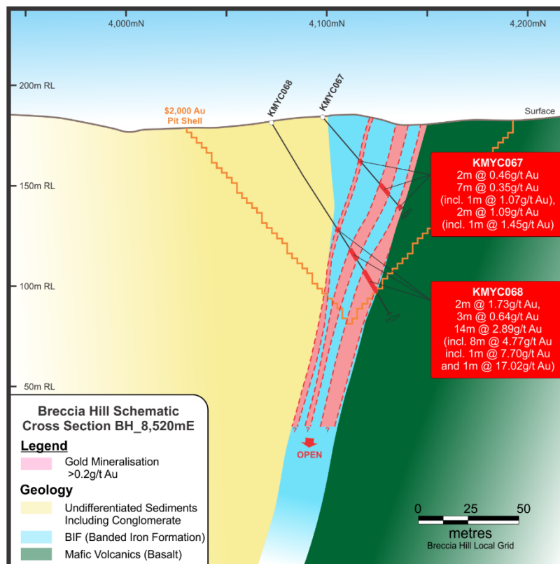
Figure 5. Breccia Hill Schematic Cross-Section, BH_8,520mE.
