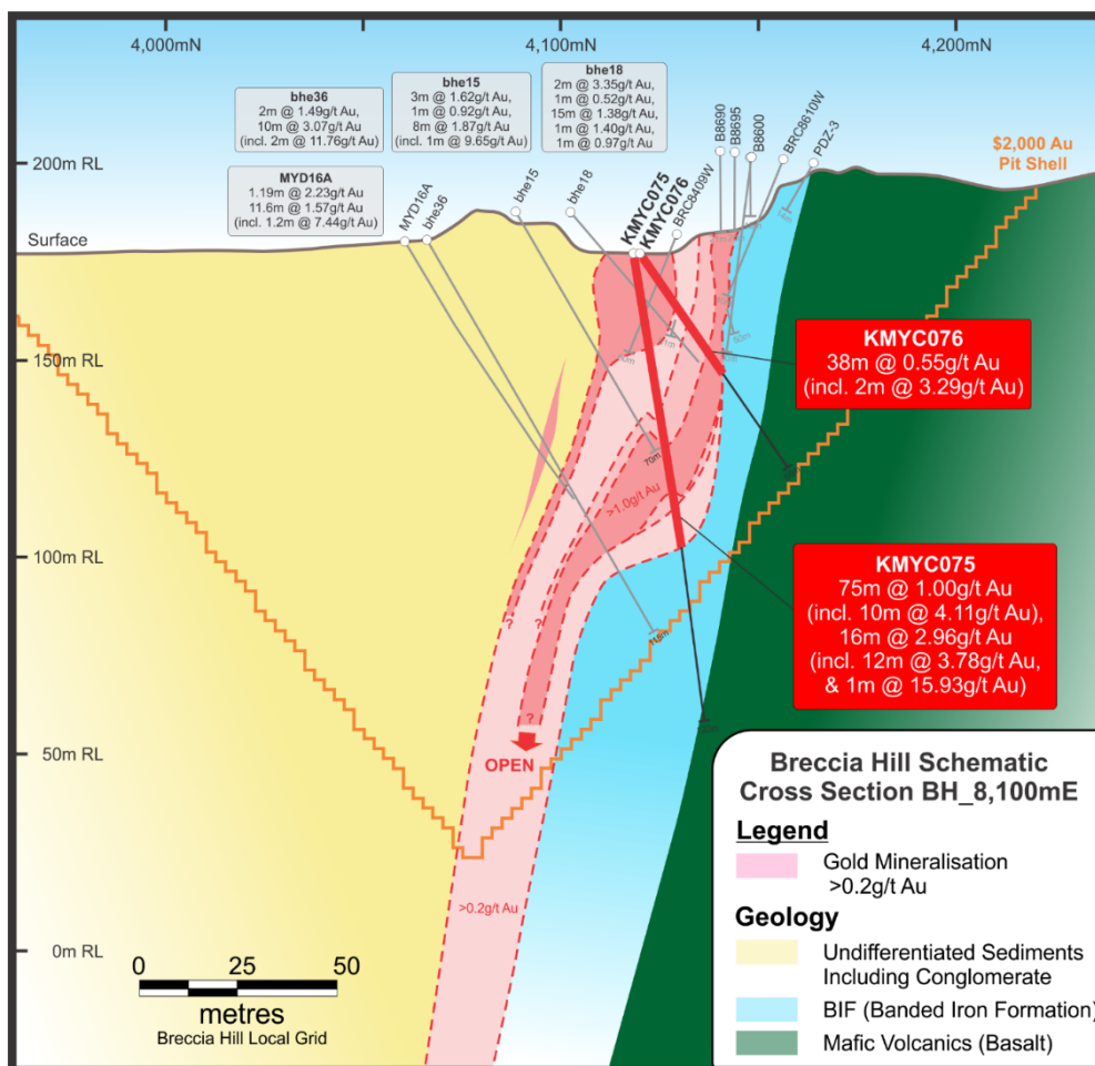
Figure 6. Breccia Hill Schematic Cross-Section, BH_8,100mE.
