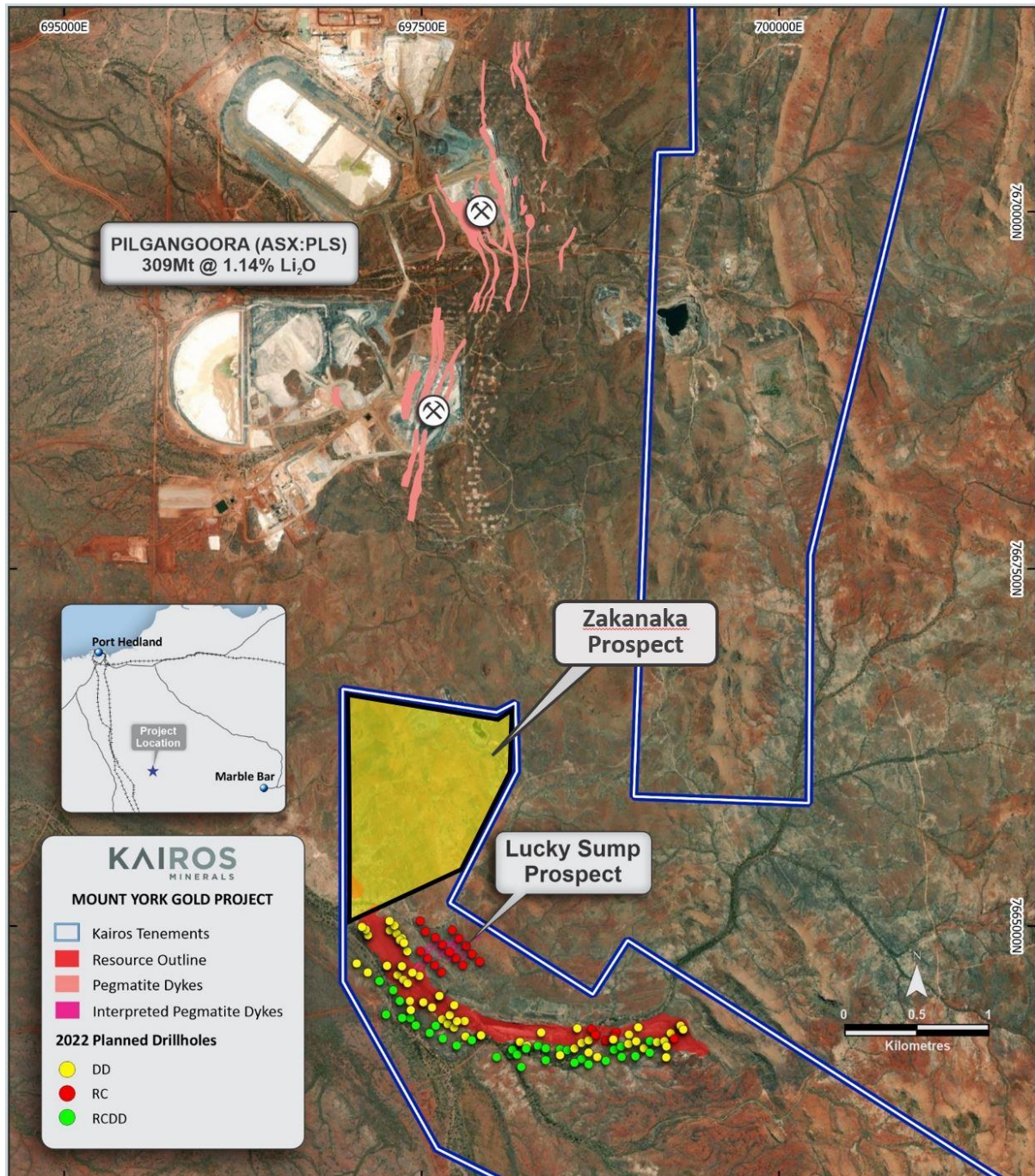
Figure 8. Lucky Sump and Zakanaka Prospect locations in relation to Pilbara Minerals' Pilgangoora's Lithium-Tantalum Mine and the Mt York Gold Project (red polygon is the Main Trend gold mineralisation).
