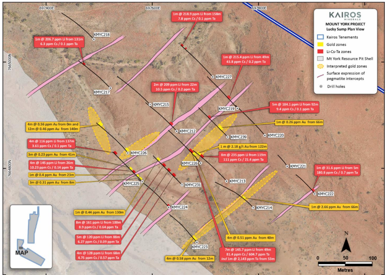
Figure 9. Lucky Sump best drill results on a plan map showing lithium-tantalum and gold intercepts from all 18 RC drill holes.
