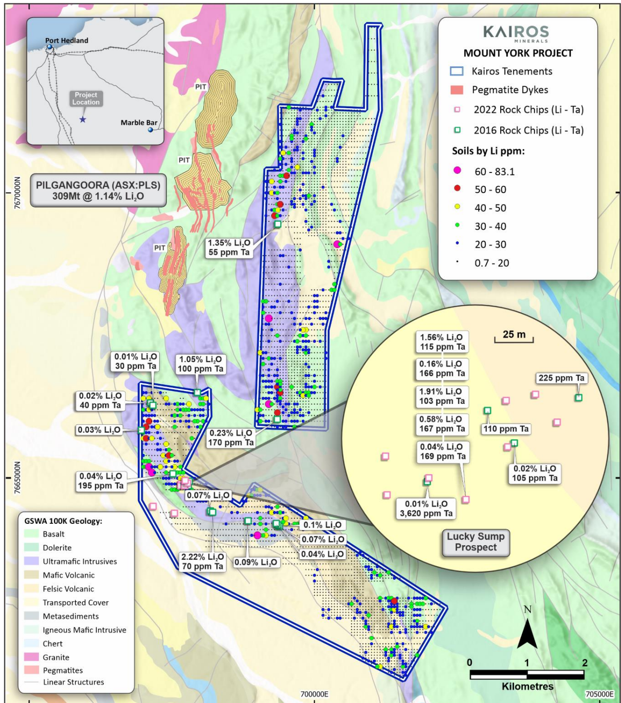
Figure 10. Lithium soil sample results from Kairos 2021 regional sampling program that were previously released for gold only (see release dated 24 September 2021). Rock chip sample results for Lucky Sump (inset) were previously reported to the ASX on 01 August 2022. Regional rock chip sample results were previously reported to the ASX on 07 June 2017.
