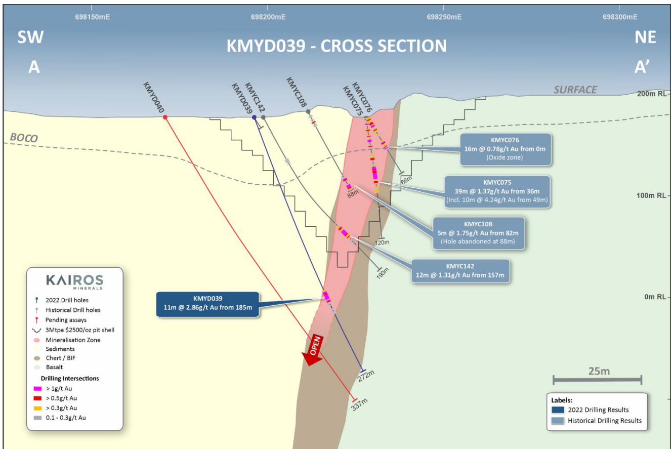
Figure 3. Breccia Hill Cross-section @KMYD039 & KMYD040. See Fig 1 for section location.
