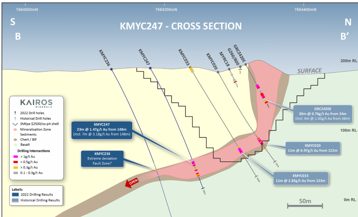
Figure 4. Gossan Hill Cross-section @KMYC247 and KMYC236. See Fig 1 for section location.
