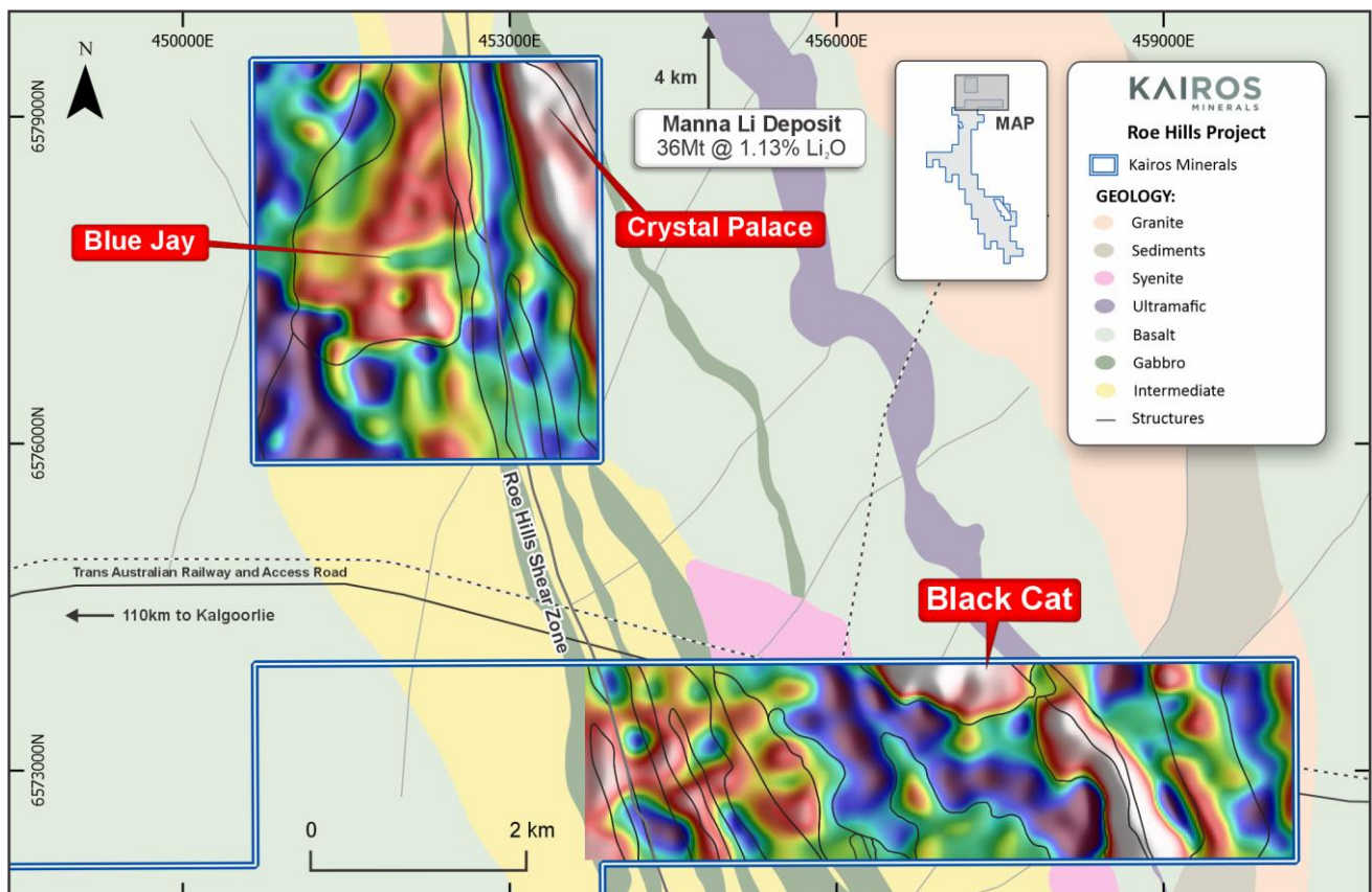
Figure 1: Roe Hills North project area showing the location of the recent 200m x 50m spaced ground gravity survey. The gravity image displayed is the first vertical derivative Bouguer anomaly with a non-linear colour stretch. Gravity lows are represented by deep blues and are generally interpreted to be potential intrusions.
