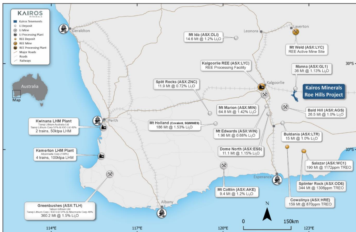
Figure 3. Location of the Roe Hills project in relation to infrastructure and other known REE and Lithium deposits and process facilities.
