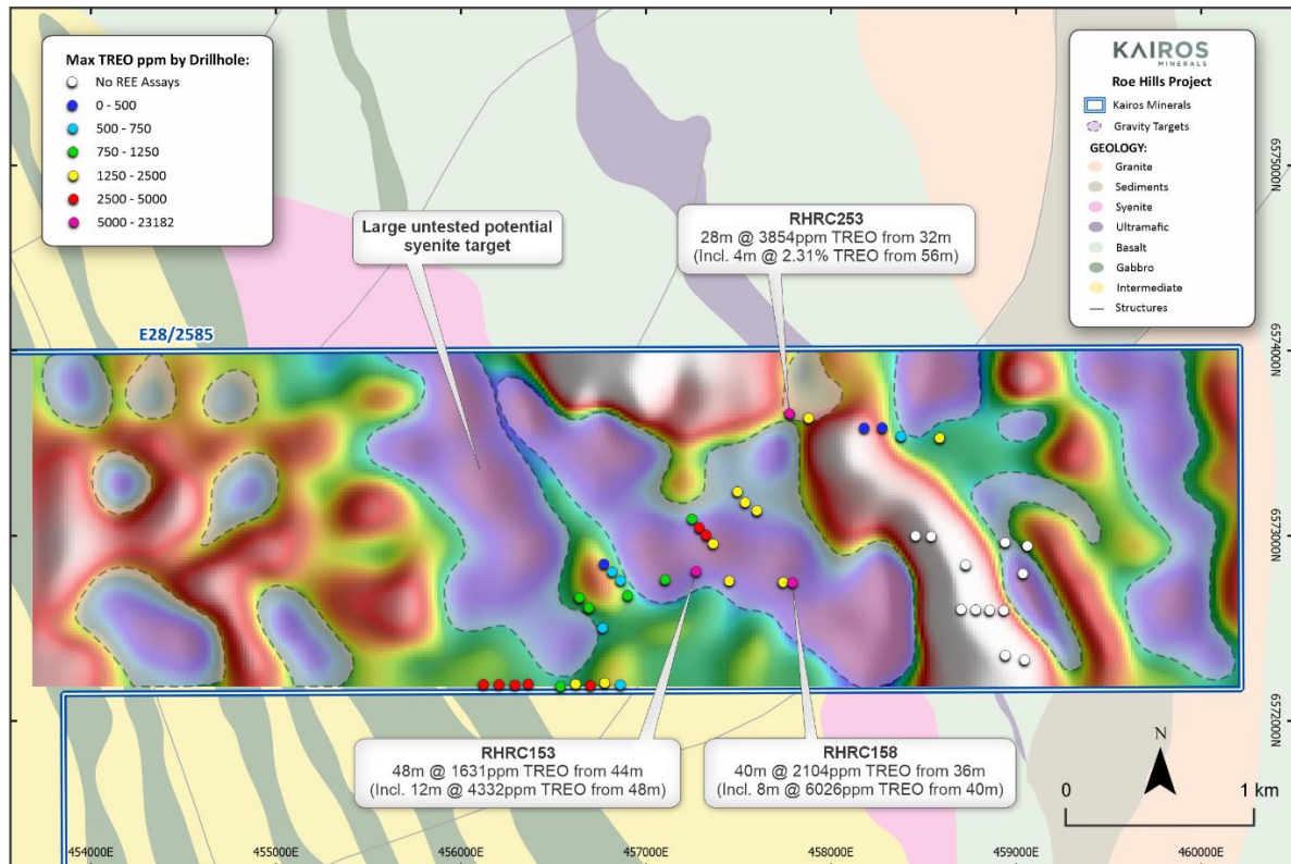
Figure 2: Black Cat area showing the location of previous drilling coloured by maximum TREO values in hole. Significant gravity lows can be observed that have not yet been drill tested. The gravity image displayed is the first vertical derivative Bouguer anomaly with a non-linear colour stretch.
