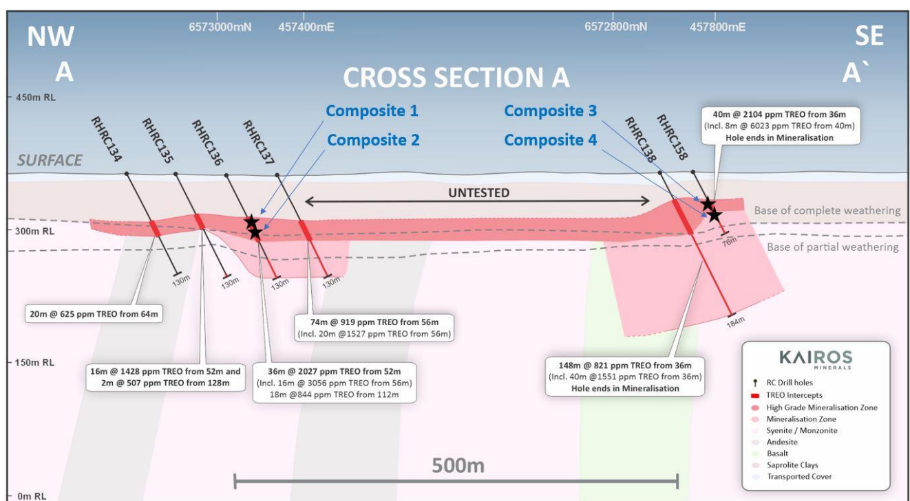
Figure 4: Cross-section through the Black Cat REE deposit showing the location of metallurgical samples collected and submitted for size analysis and leach testing.
