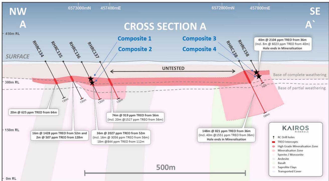
Figure 3: Cross-section through the Black Cat REE deposit showing the location of metallurgical samples collected and submitted for size analysis and leach testing.
