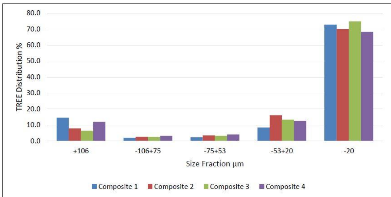
Figure 4. TREE distribution within each size fraction of each composite sample.
