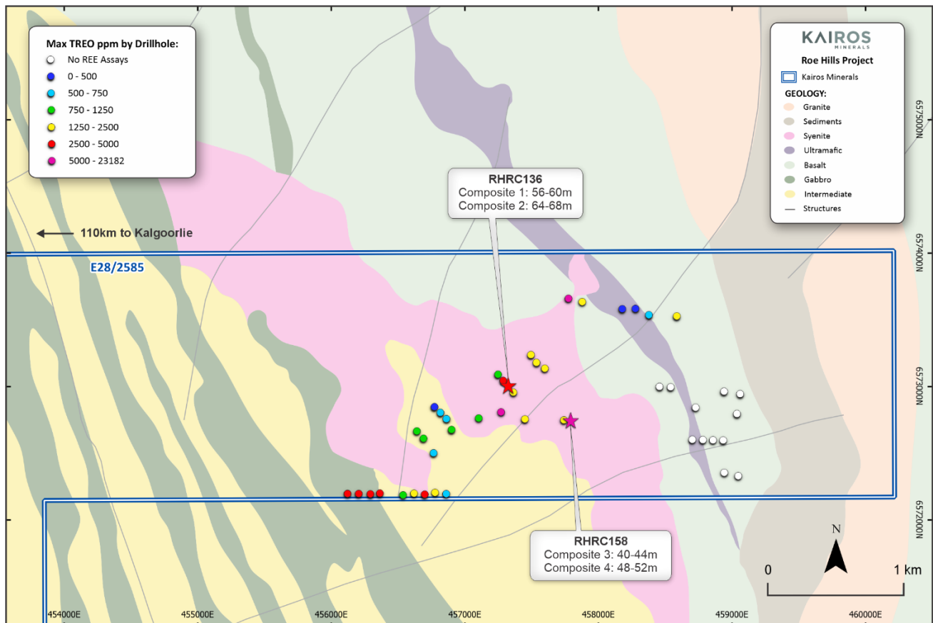
Figure 2: Geology interpretation from drilling data and gravity surveying of the Black Cat REE deposit showing the location of drillholes RHRC136 and RHRC158 from which metallurgical samples were selected and submitted for size analysis and leach testing. The pink indicates the potential ore-source syenites interpreted from the gravity survey that provides significant untested drill targets for future aircore drilling.
