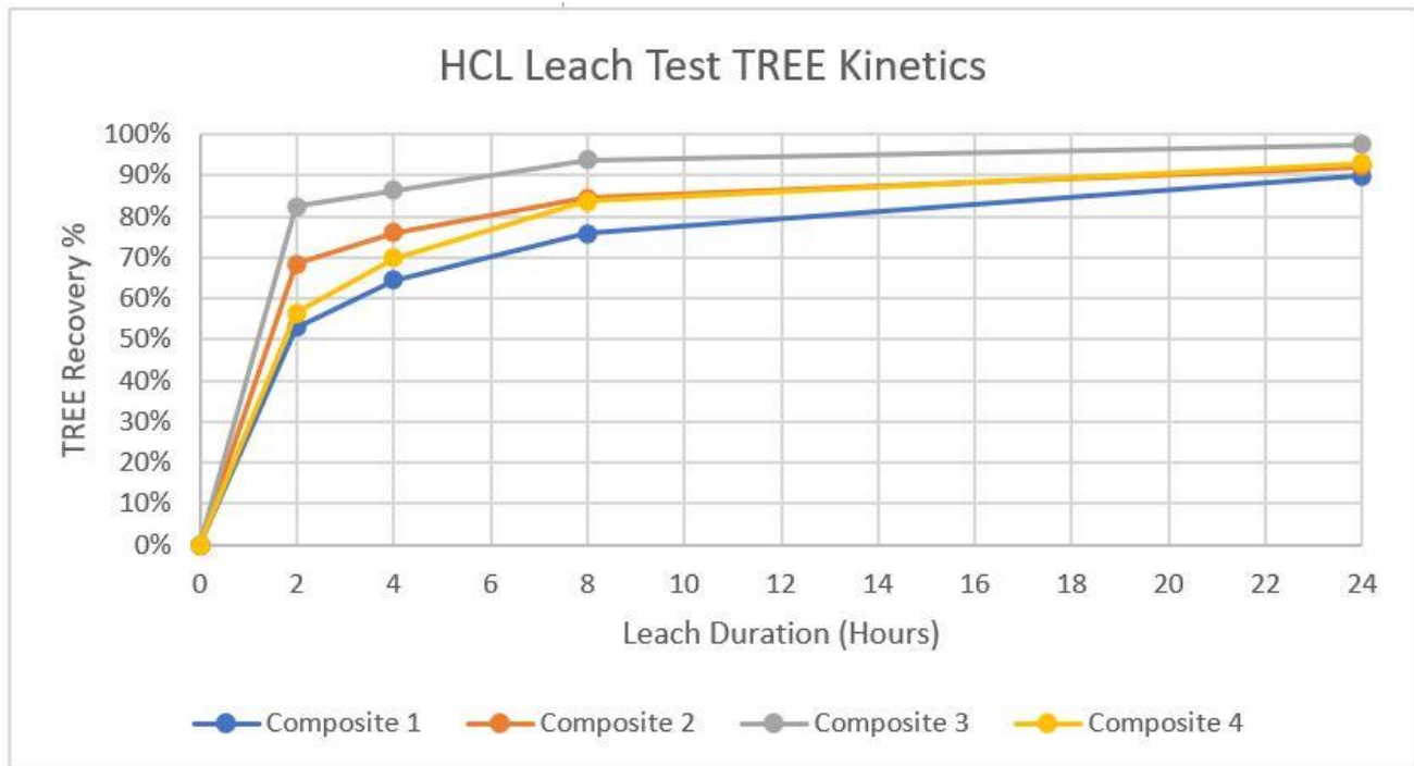
Figure 7. Chart showing leach test results for four composite samples from Black Cat in HCl at 25g/L concentration and 50°C temperature over 2, 4, 8 and 24 hours.
