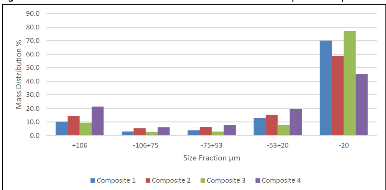
Figure 5. Mass distributions of size fractions for each composite sample.
