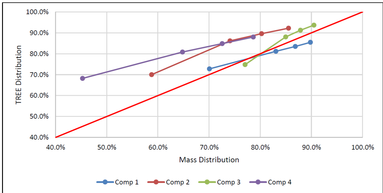
Figure 6. Composite Mass versus TREE distribution. Composites 2 and 4 show a positive trend of ‘enriched’ TREE distribution relative to their Mass distribution and could be considered encouraging results for possible beneficiation through sizing.
