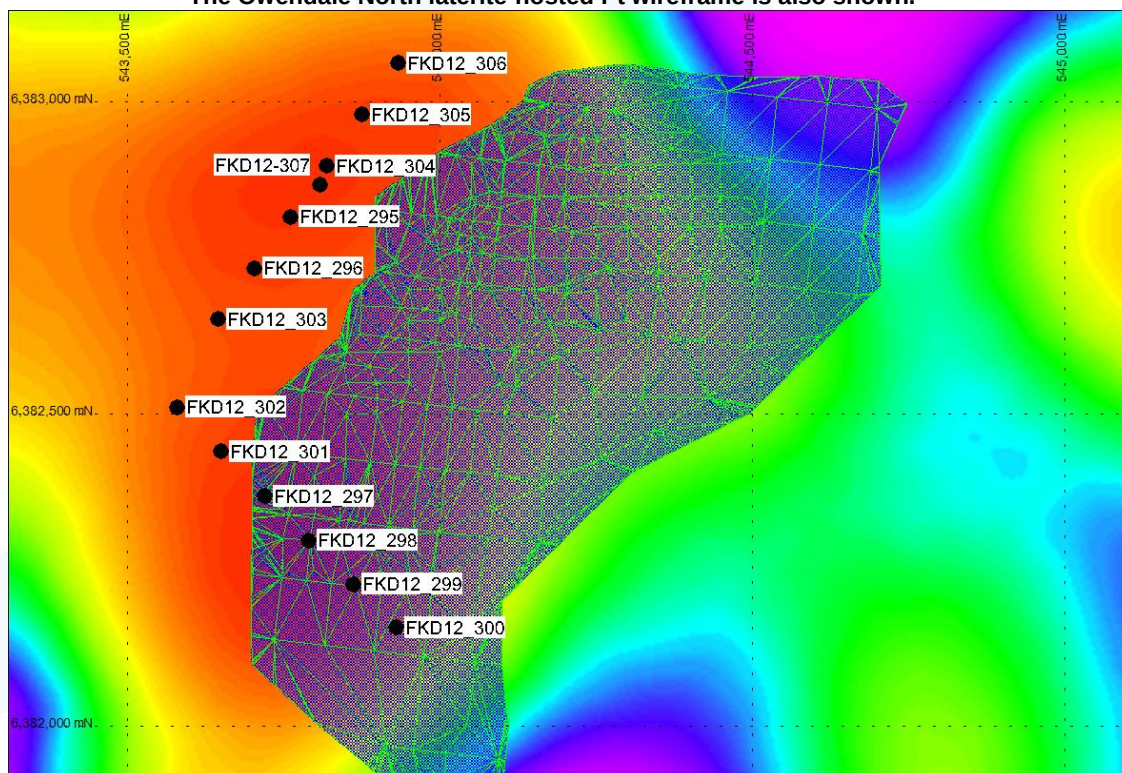
Figure 2. Location map for drill-holes targeting primary Pt mineralisation. The background image is Induced Polarisation intensity (warm colours are more intense, and vice versa). The Owendale North laterite-hosted Pt wireframe is also shown.
