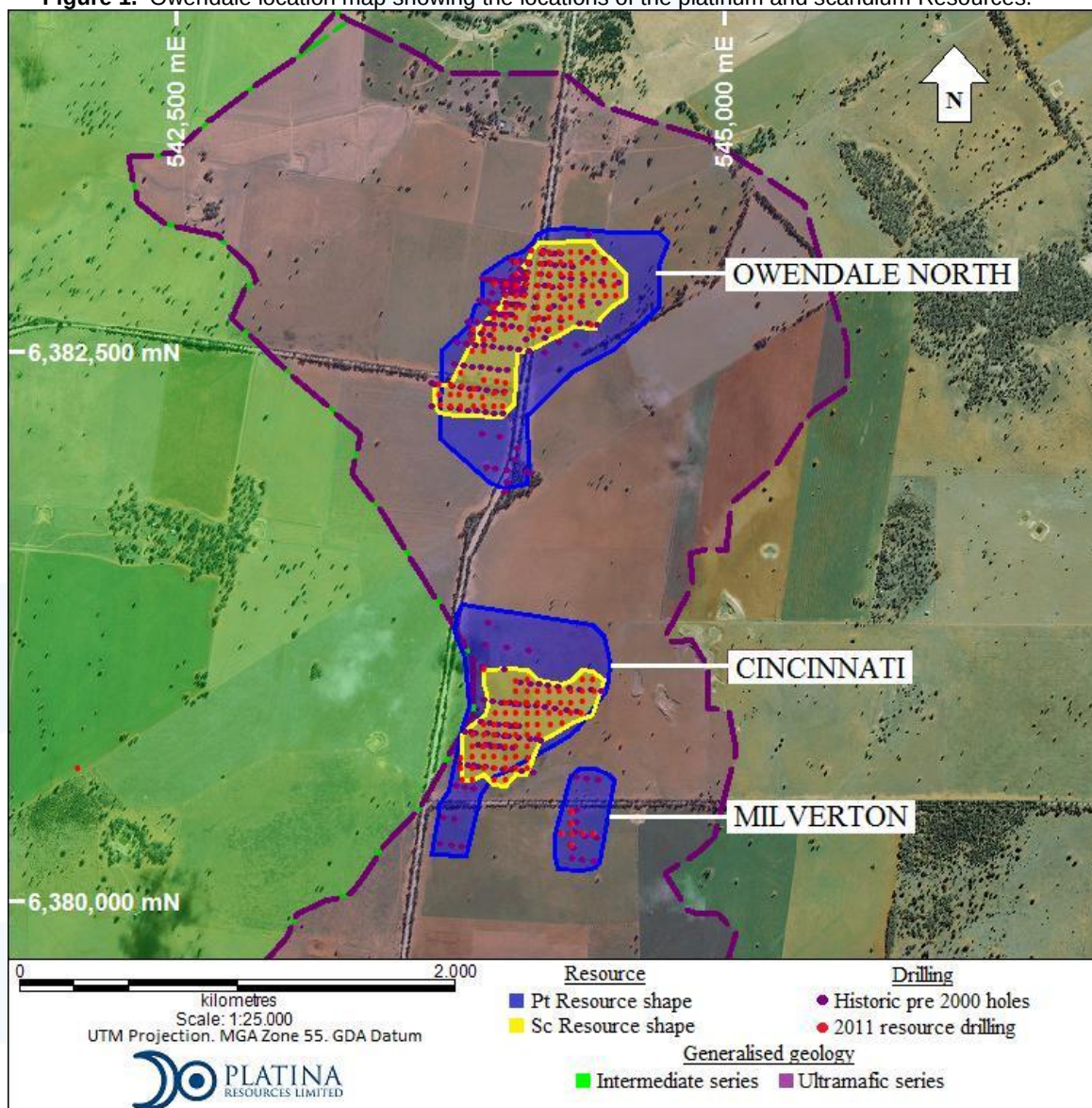
Figure 1. Owendale location map showing the locations of the platinum and scandium Resources.
