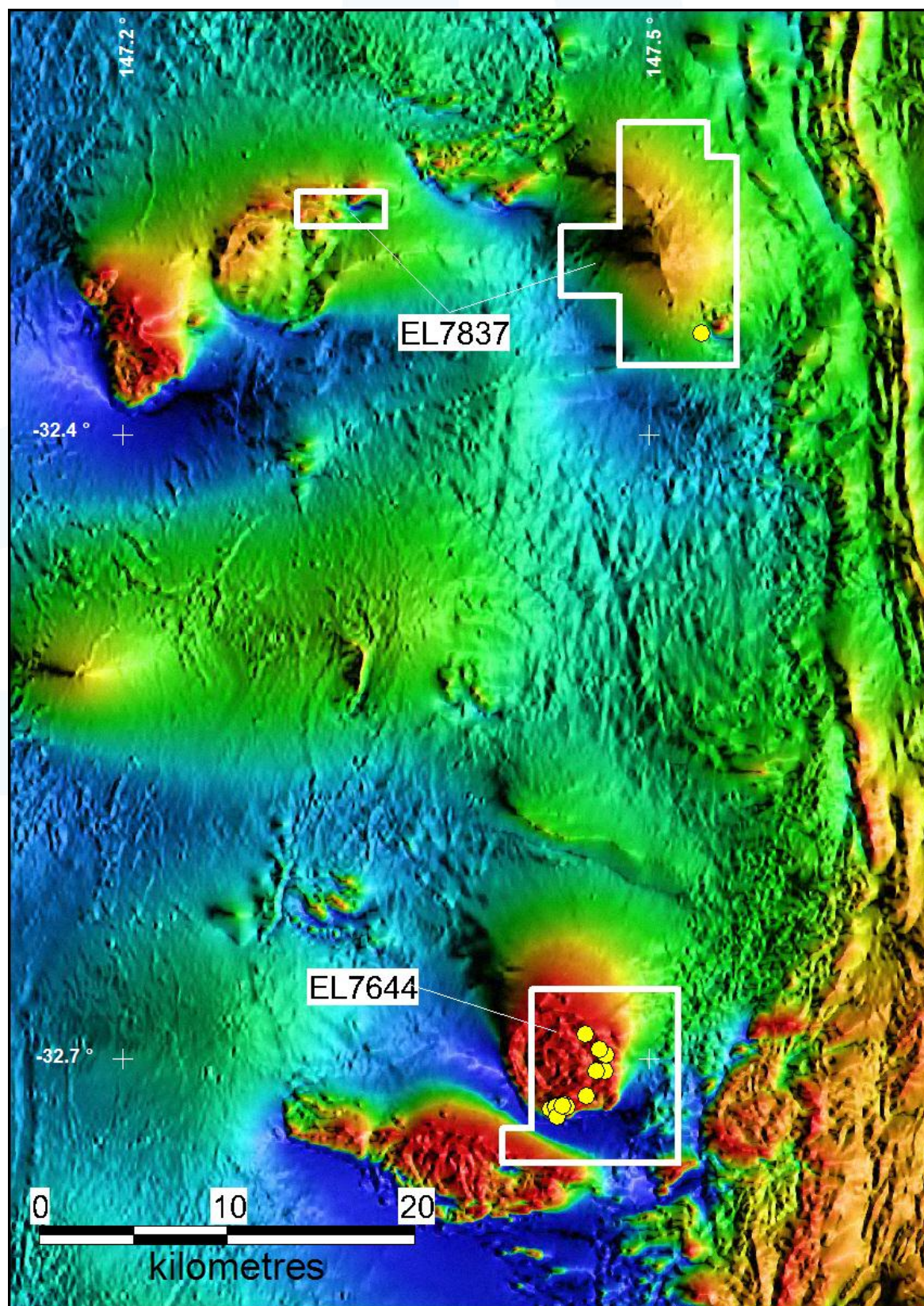
Figure 1. Drill-hole location map for EL7837 & EL7644 (Owendale). Drill-holes are shown as yellow dots. Background image is regional total magnetic intensity.
