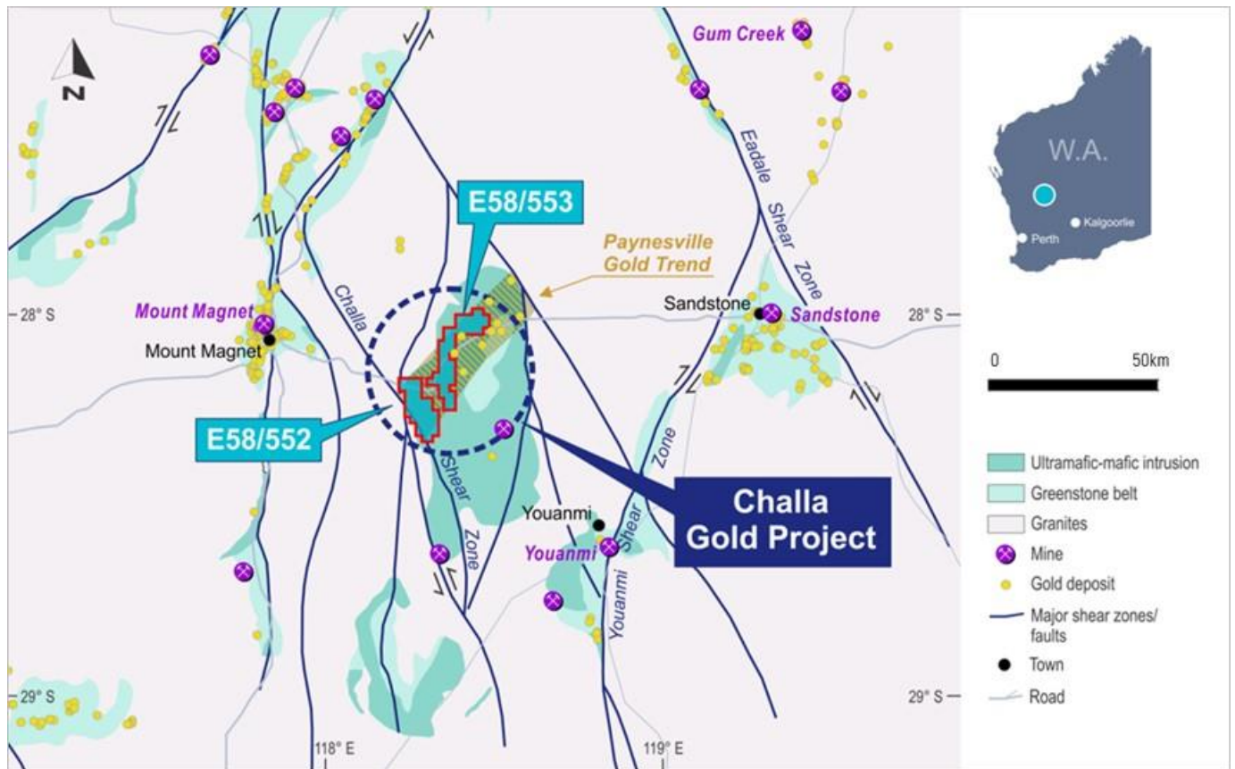
Figure 3: The Challa Gold Project lies in-between the prolific Mt Magnet and Sandstone gold districts in Western Australia at the southwest end of the recently identified Paynesville Gold Trend.
