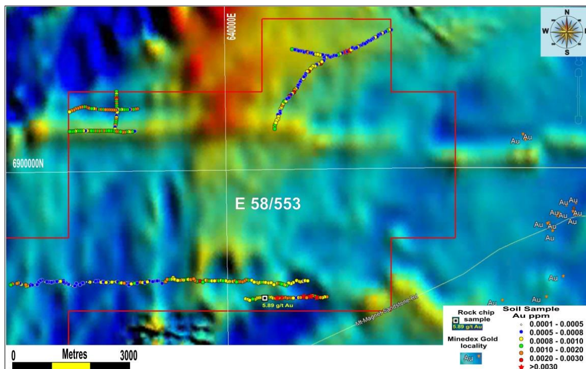
Figure 1: Soil sampling results - E 58/553
