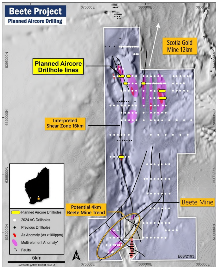
Figure 3. Map showing plan view of the planned AC holes' location at the Beete Project. Also showing May-June 2024 aircore drill holes and generated targets over GSWA's reprocessed TMIRTP WA State merged magnetics
