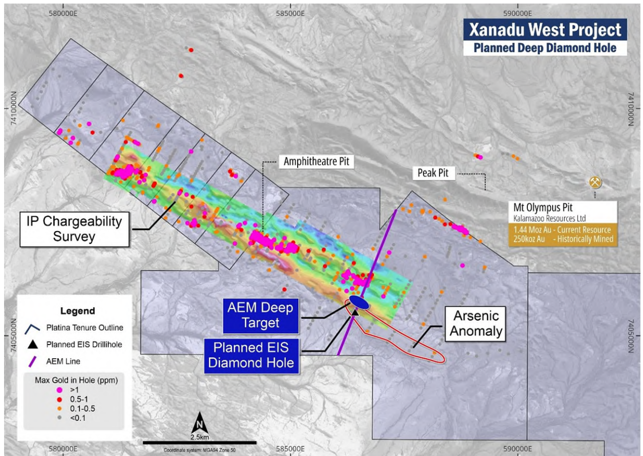
Figure 6. Plan view of the Xanadu West area with max gold in hole over IP chargeability, tenure and google satellite image.
