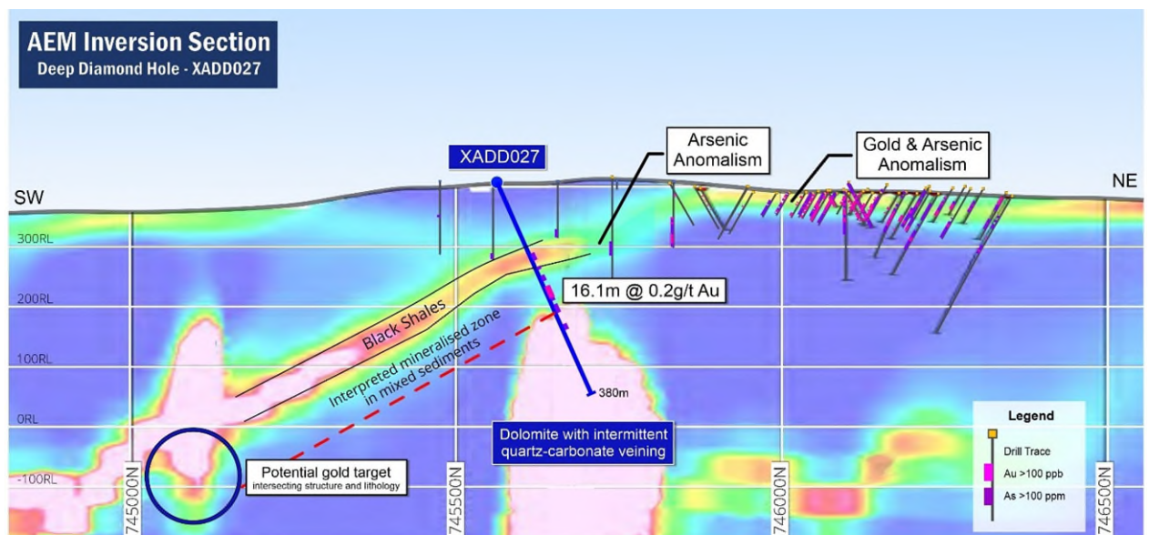
Figure 5. Section across XADD027 with new assay results and interpretation which lies south of the Cleopatra prospect. Section limits +/-200m. Section showing the aero electromagnetic one-dimensional inversion scheme interpretation done by Southern Geoscience in 2021. The original survey on the line 2024002 Bearing 030 was flown by AusAEM 02 WA/NT in 2019-20.
