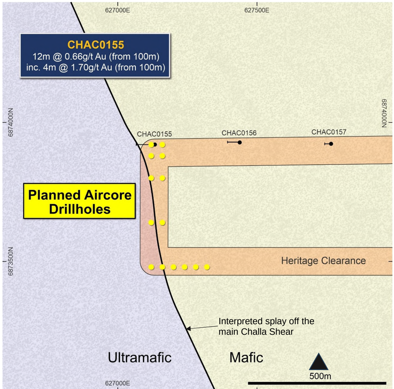
Figure 2. Map showing plan view of the planned AC holes at the Challa Project. Also showing July-August 2024 aircore drill holes overlaying heritage clearance area and interpreted geology from AC drilling.
