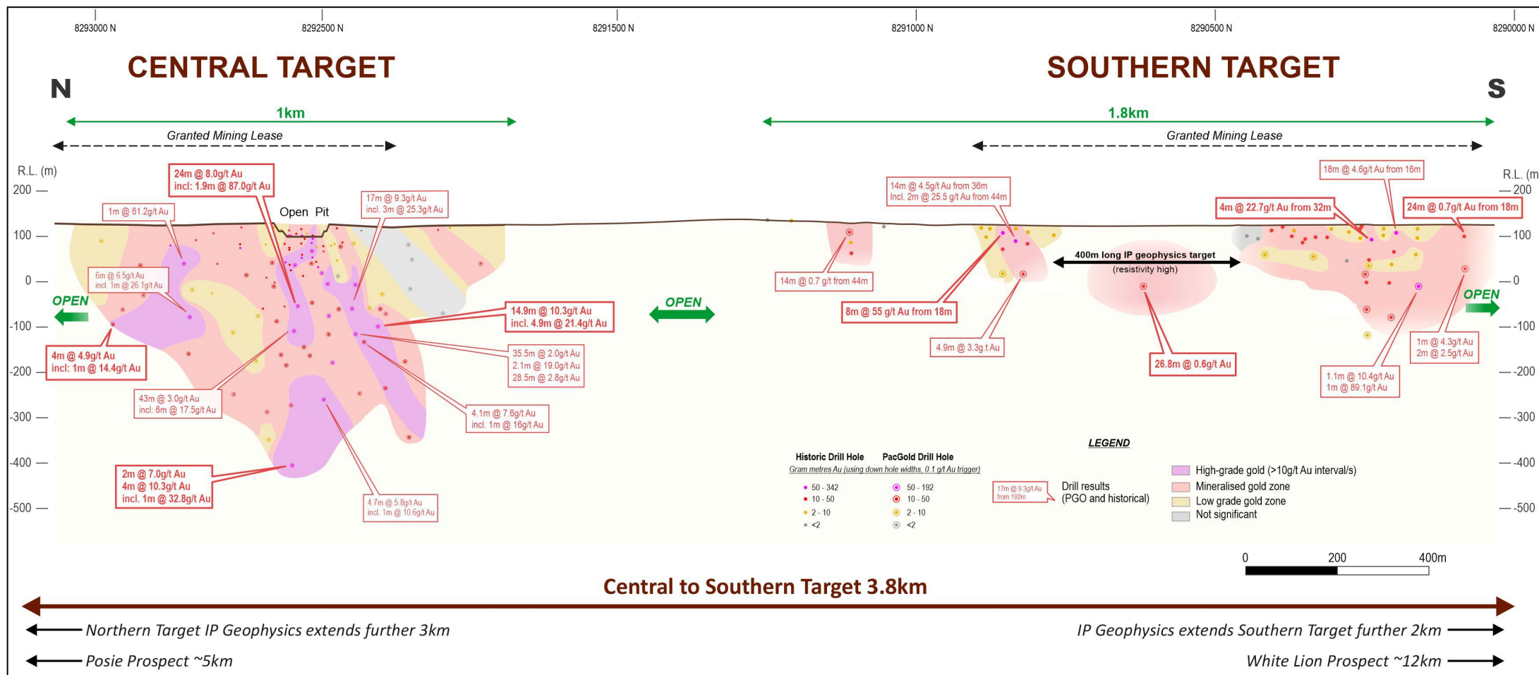
Figure 3: Central to Southern Target long section highlighting over 3.8km of strike (open) demonstrating large-scale gold system
