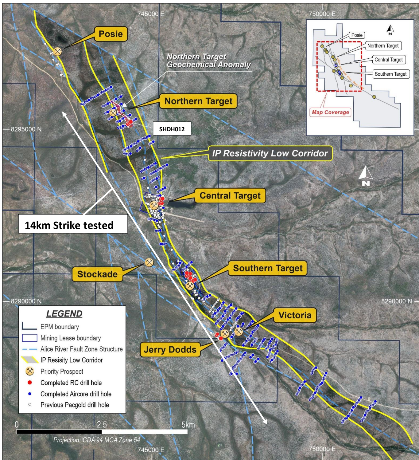
Figure 1: Completed Aircore and RC holes from current program. The IP geophysical corridor shown in yellow over a strike extent in excess of 15km
