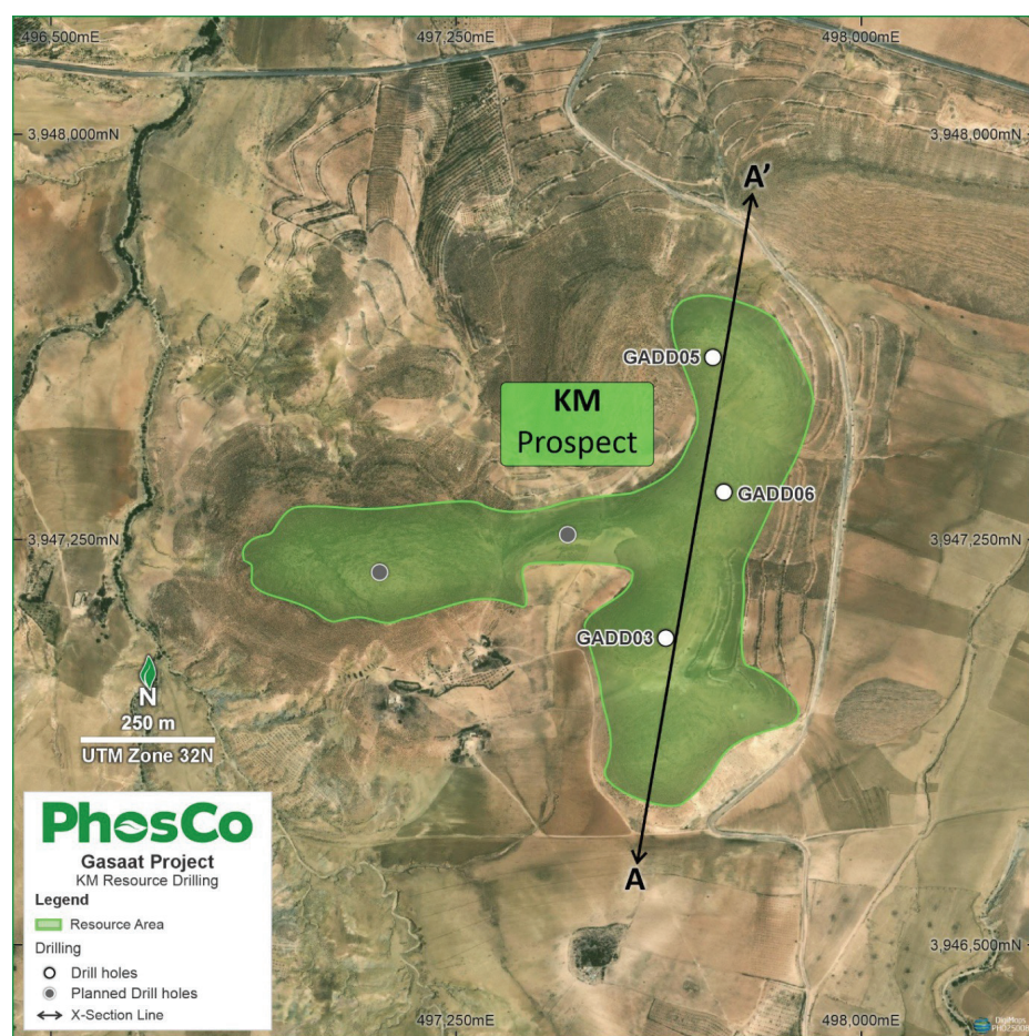
KM Prospect showing location of Section A-A' and planned drill holes
