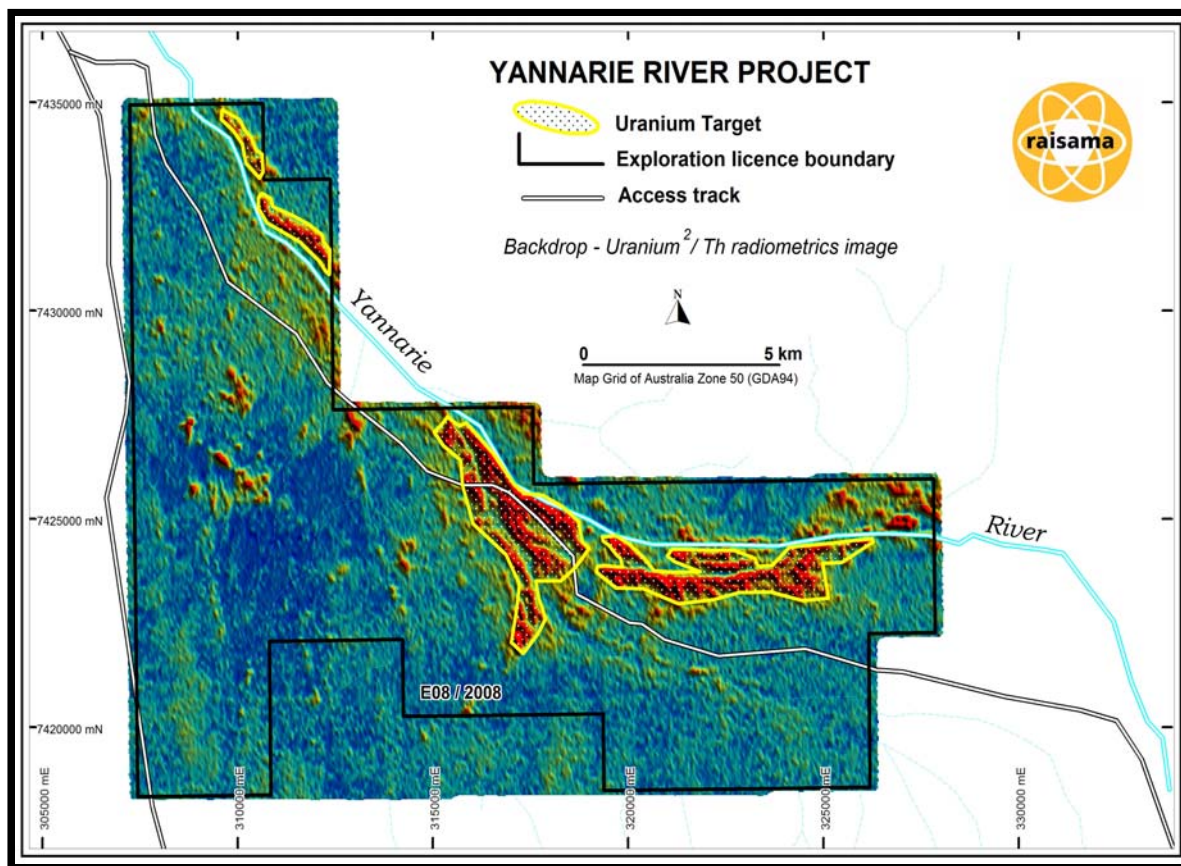
Figure 1: Uranium targets on uranium 238 / thorium radiometric image
