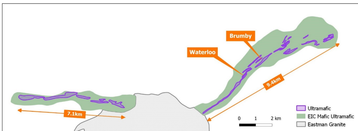
Figure 2. Location of the Brumby and Waterloo Prospects within the Eastman Intrusion.
