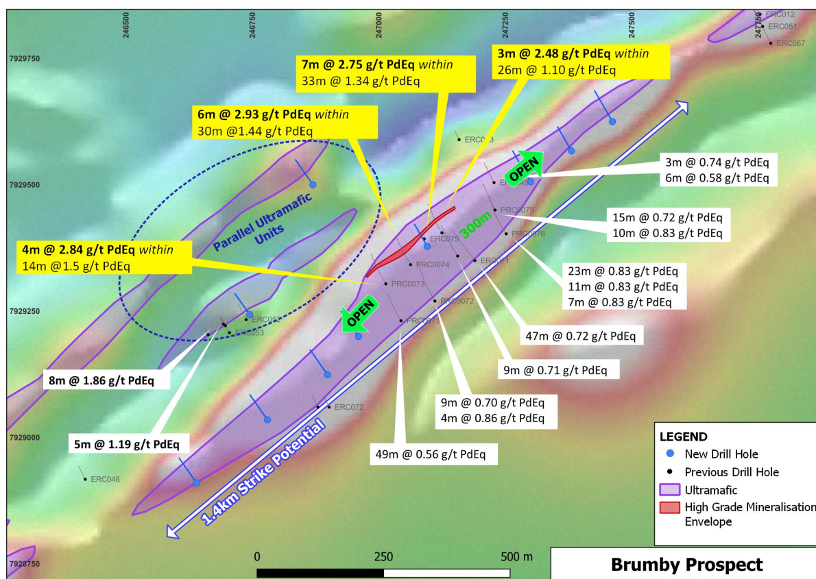
Figure 3. Brumby Prospect showing previous drill results over an interpreted Ultramafic intrusion draped over a background aeromagnetic image. The latest completed drillhole traces are shown in blue.
