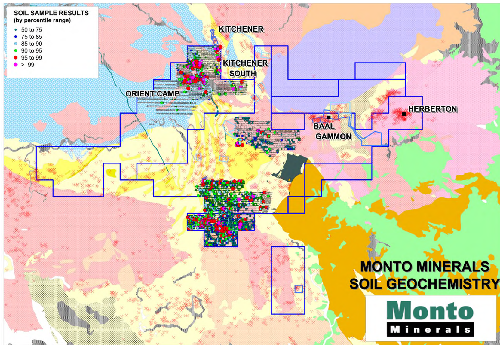
Figure 3: Herberton Project Soil Geochemical Survey to Date showing the Kitchener South and Orient Camp Zones
