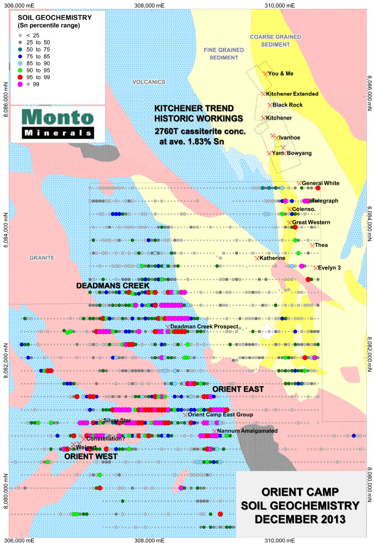
Figure 4: Soil Geochemistry – Orient Camp (West and East) and Kitchener Trend Anomalies
