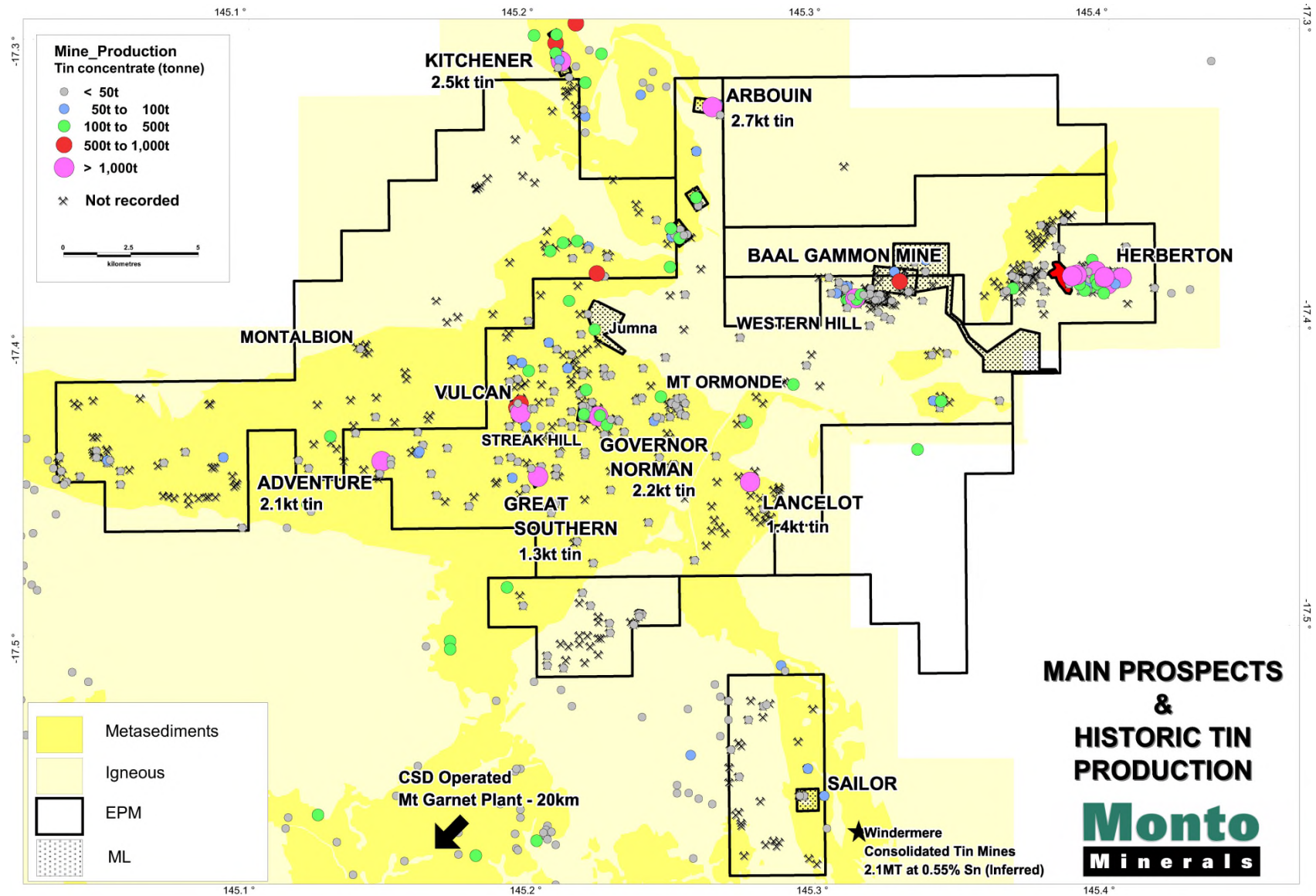
Figure 1: Herberton Project – Main Prospects and Historic Mines
