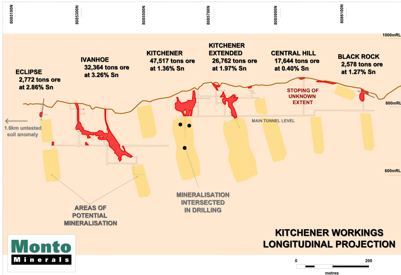
Figure 2: Kitchener Workings - Long Section
