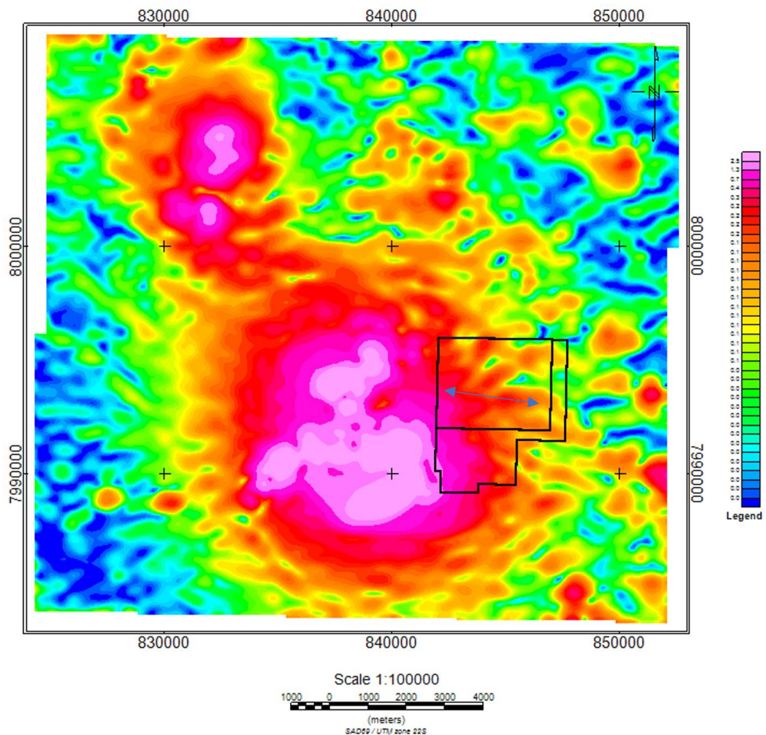
Figure 4. Magnetic survey showing prominent east west structure next to CMOC niobium mine
