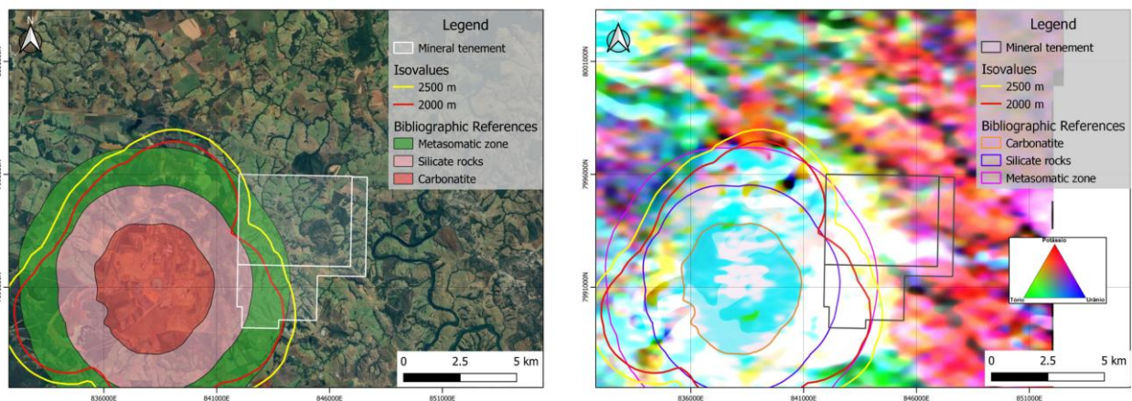
Figure 1. The above schematics (1a and 1b) produced by GE21, our geological consultants show the concession outline in white and the prominent east west structure. The metasomatic zone is the key area for ionic clays and the right hand side schematic (1b) shows uranium in blue, thorium in green and potassium in red from the radiometric survey.
