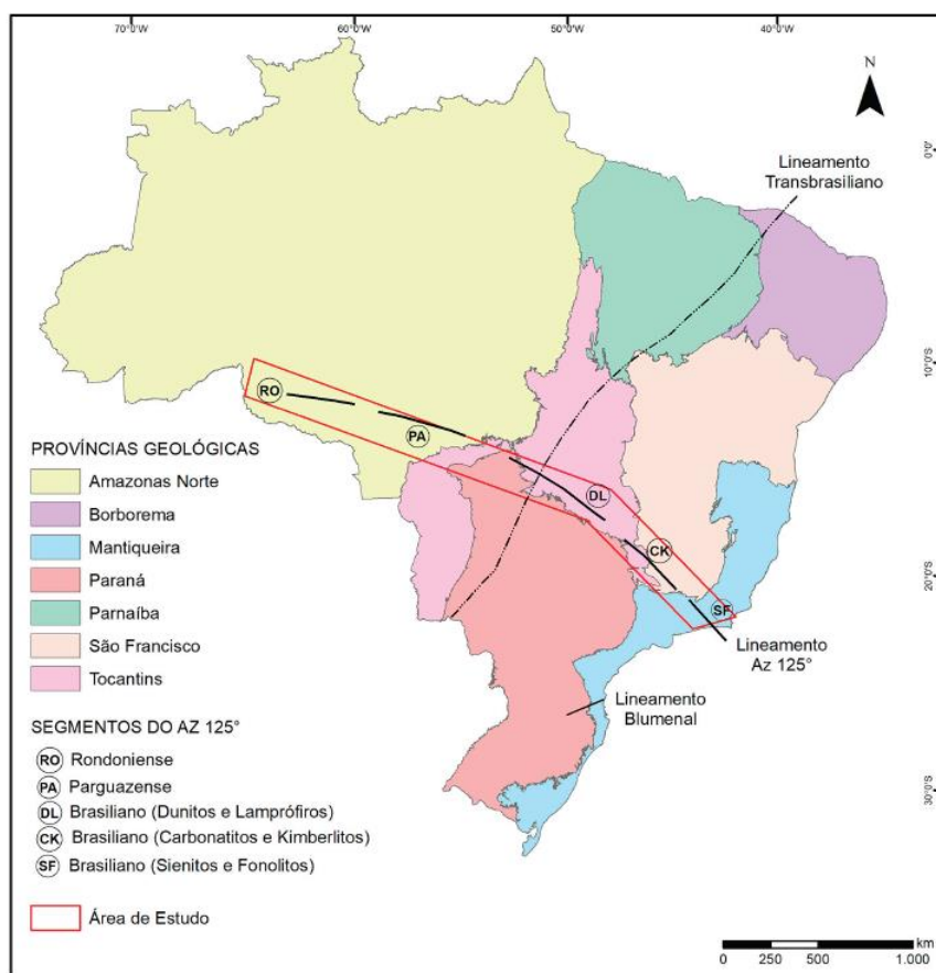
Figure 6. Araxá and Catalão 1 Rare earth mines (CK) are on the same trend, 125 AZ . The bibliographic references show the same genesis and geological event as observed in Goais.
