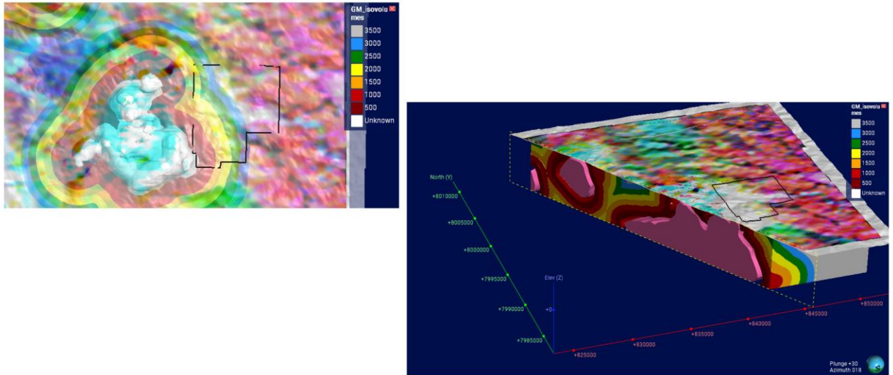
Figure 8. Shows magnetic inversions and distances derived by AI models of existing deposits and a section of what the body looks like from references and geophysics. The heat source is emanating from the bottom left hand corner at depth.
