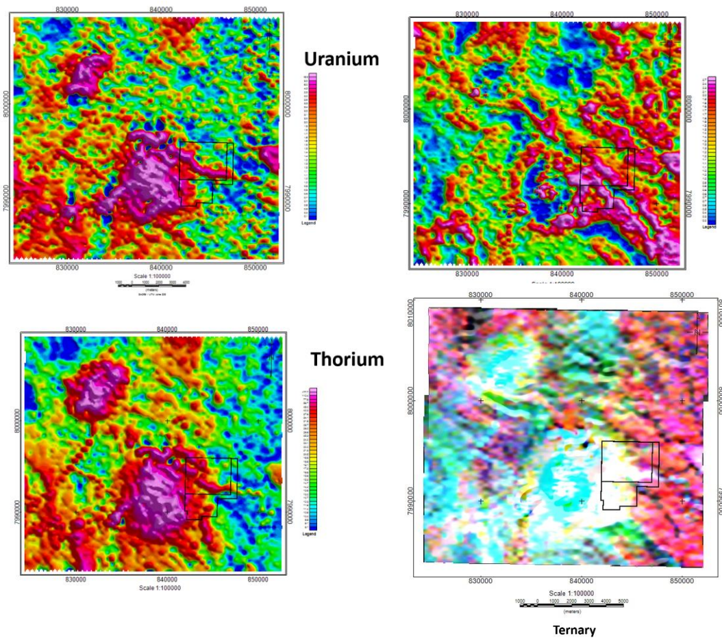
Figure 5: Shows radiometric surveys for thorium, uranium and potassium and ternary analysis showing white zones where fenitization has probably occurred.
