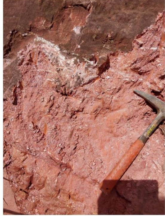
Figure 4. Fenitised Araxa shale. Metasomatic zone of chemical compositional alteration of the rock and percolation of the fluid network through the fractures when the carbonatite dome rose. Ionic clays and saprolite below the rock, prospective for REE's.
