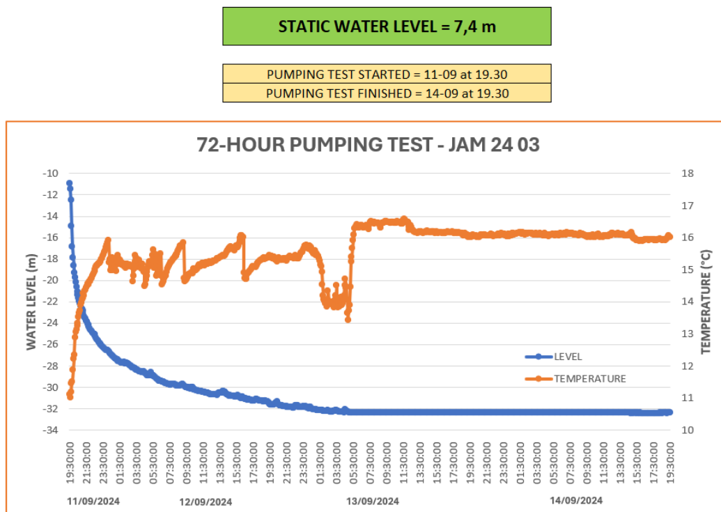
Figure 7 Aquifer test analysis - drill hole JAM-24-03.
