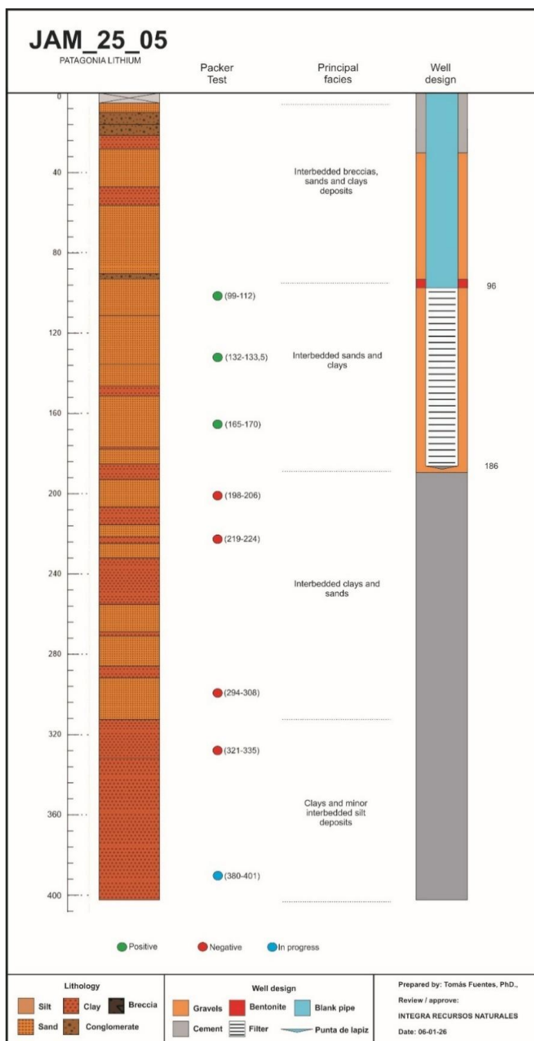
Figure 2. Schematic showing the sediments encountered to the EOH 401m depth JAM 25-05.
