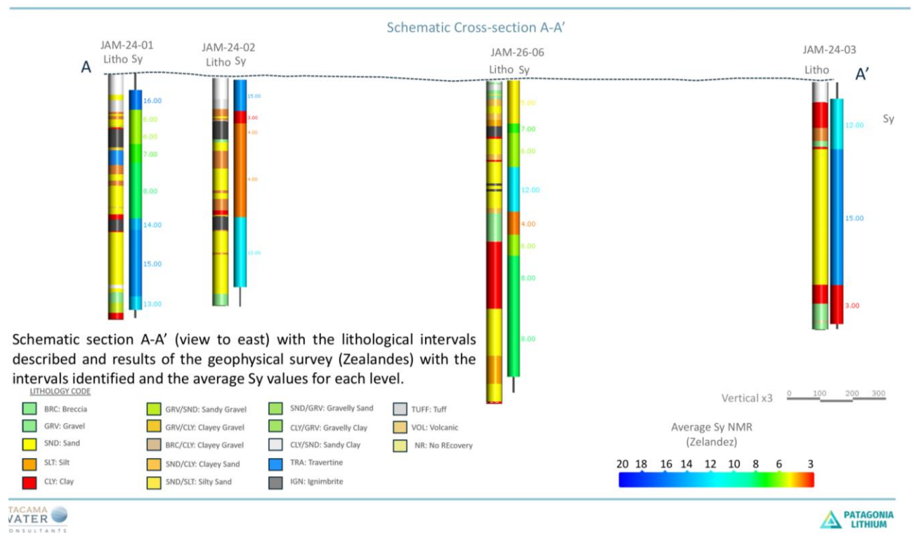
Figure 5. Section showing lithology and the high porosity as measured by specific yield - lots of green and blue.
