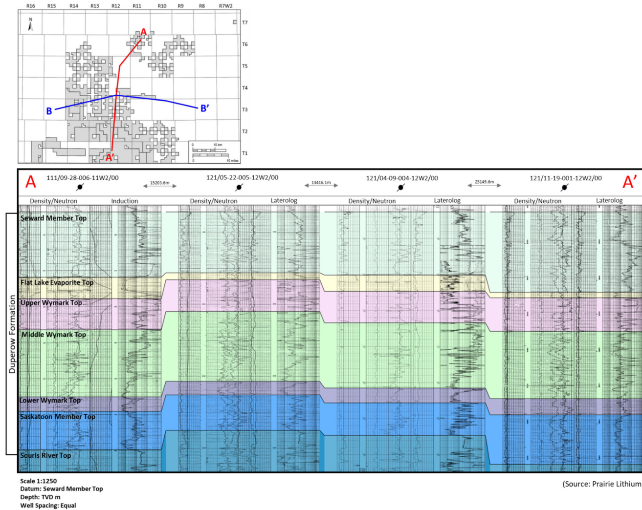
North-South Orientated Stratigraphic Cross-Section A-A' with the Top of the Duperow Formation Surface as a Datum
