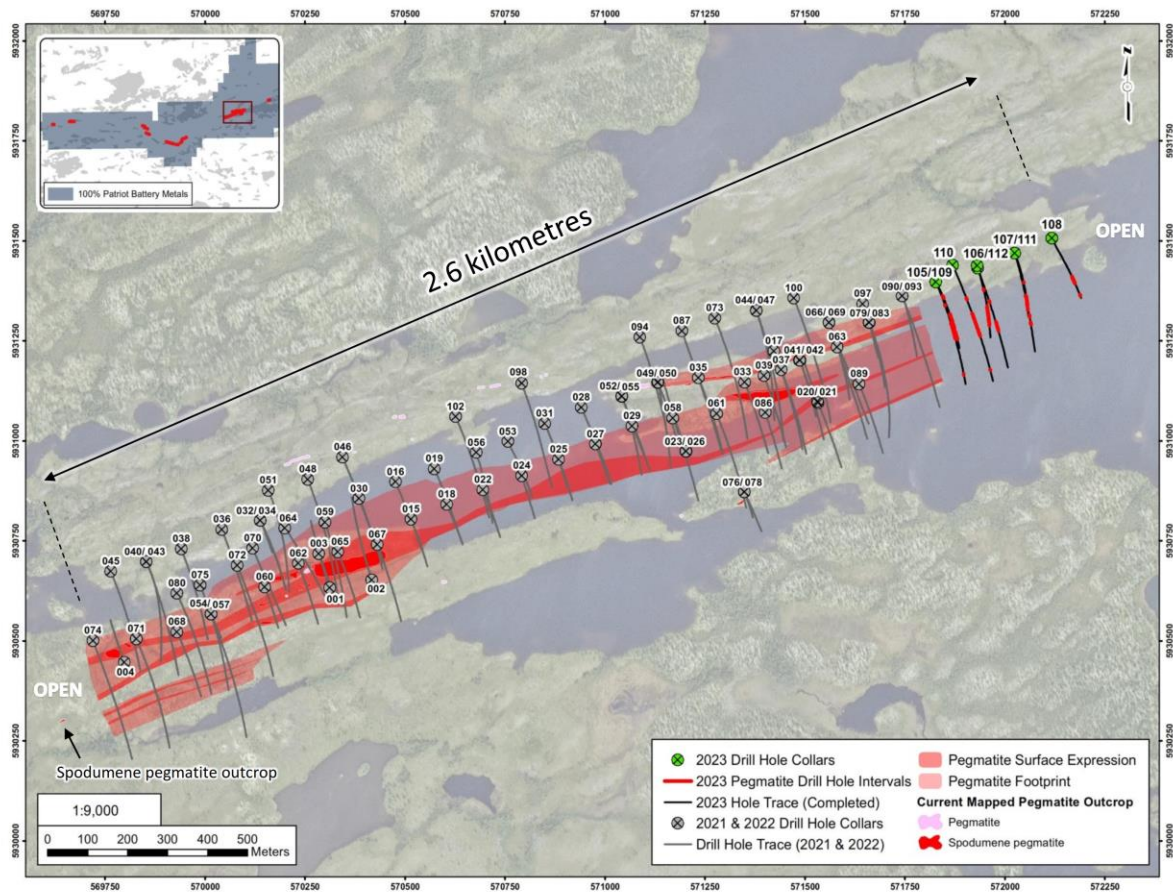
Figure 1: Drill hole locations through CV23-112 at the CV5 Pegmatite
