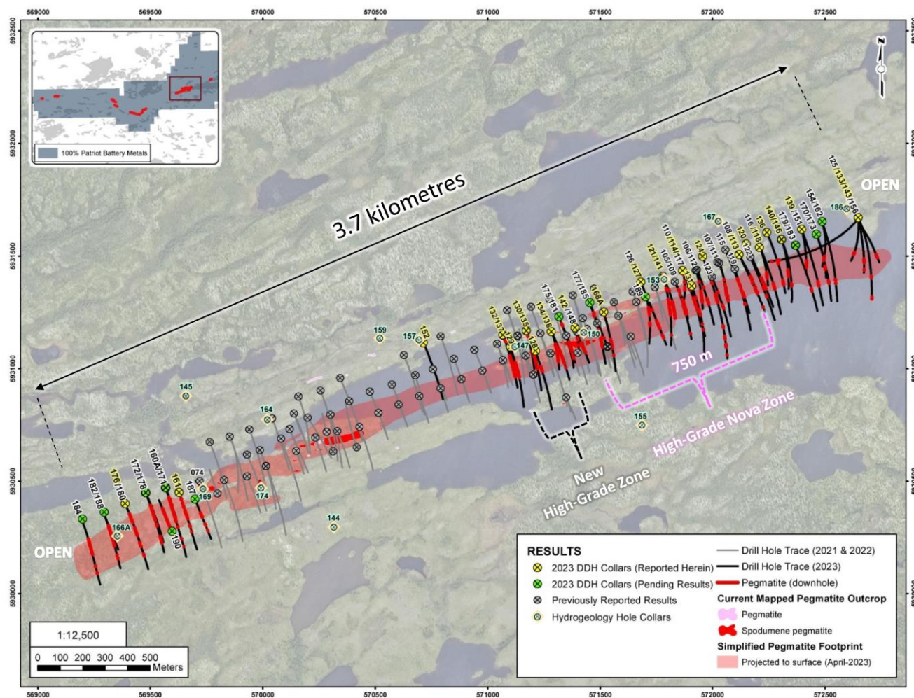
Figure 1: Drill holes completed at the CV5 Pegmatite through the 2023 winter drill program
