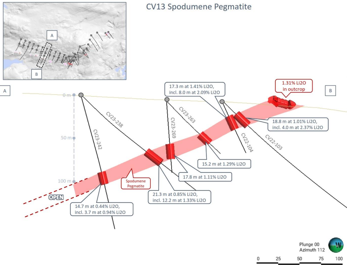
Figure 2: Cross-section of the CV13 Spodumene Pegmatite's geological model along its western arm.
