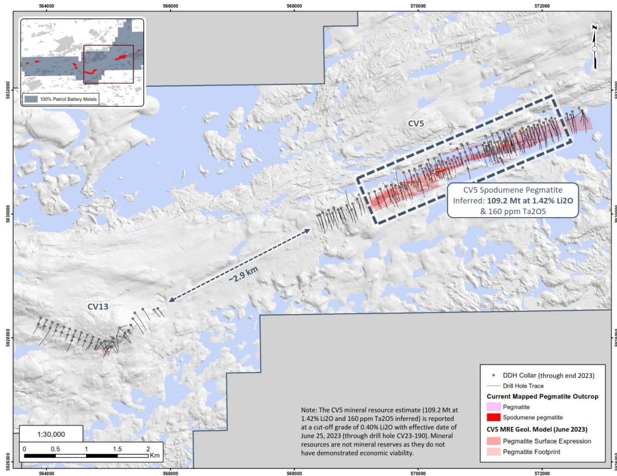
Figure 3: Corridor remaining to be drill tested between the CV5 & CV13 spodumene pegmatites.
