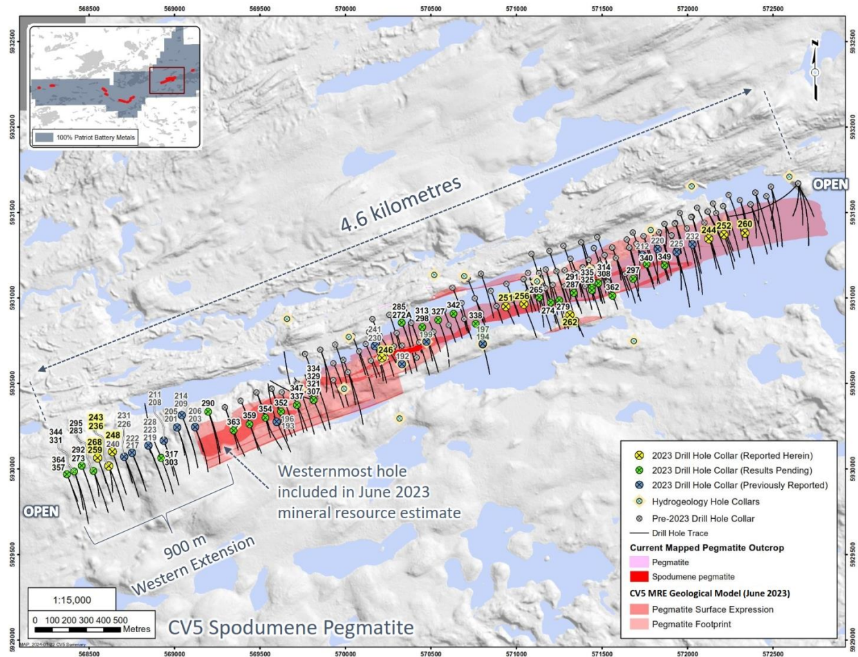
Figure 1: Drill holes completed through 2023 at CV5 Spodumene Pegmatite.
