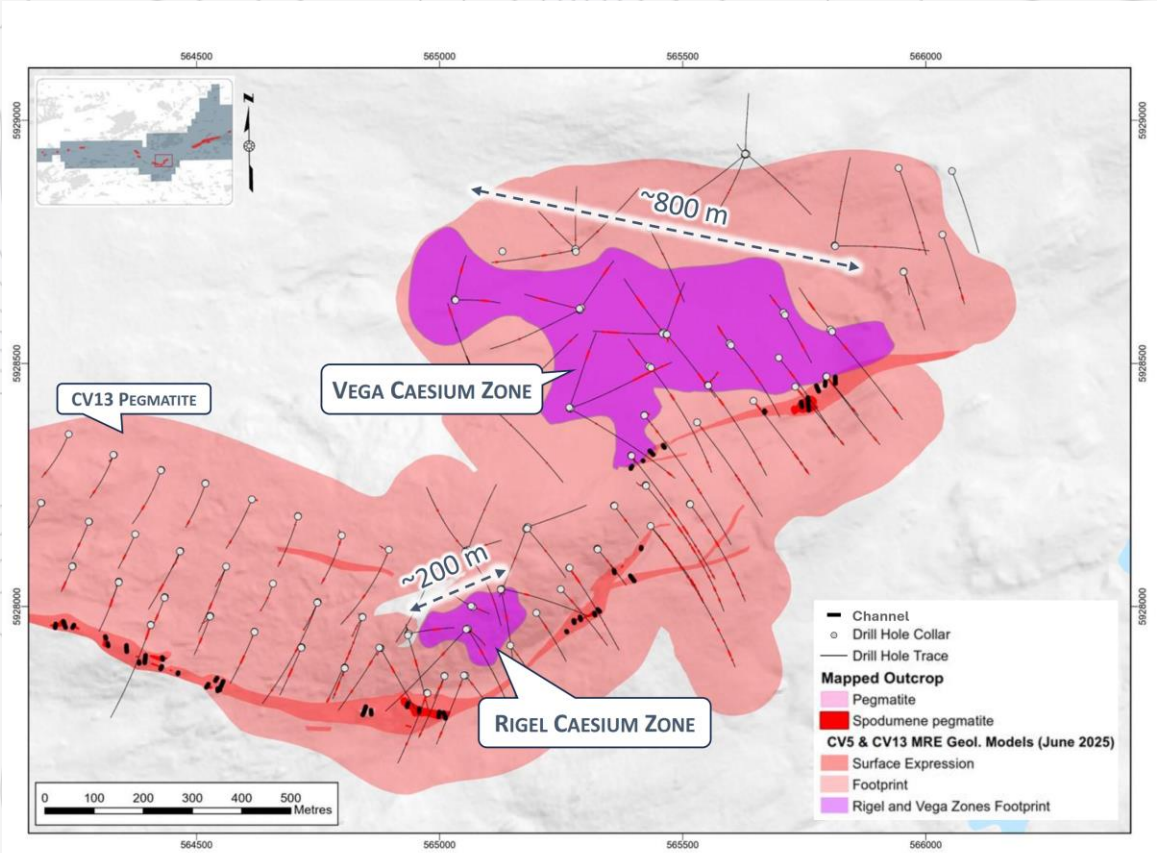
Plan view of the Vega and Rigel caesium zones based on a 0.50% Cs 2 O grade constraint within the wider CV13 Pegmatite body. Refer to news release dated July 20, 2025 "World's Largest Pollucite-Hosted Caesium Pegmatite Mineral Resource Defined at Shaakichiwaanaan"
