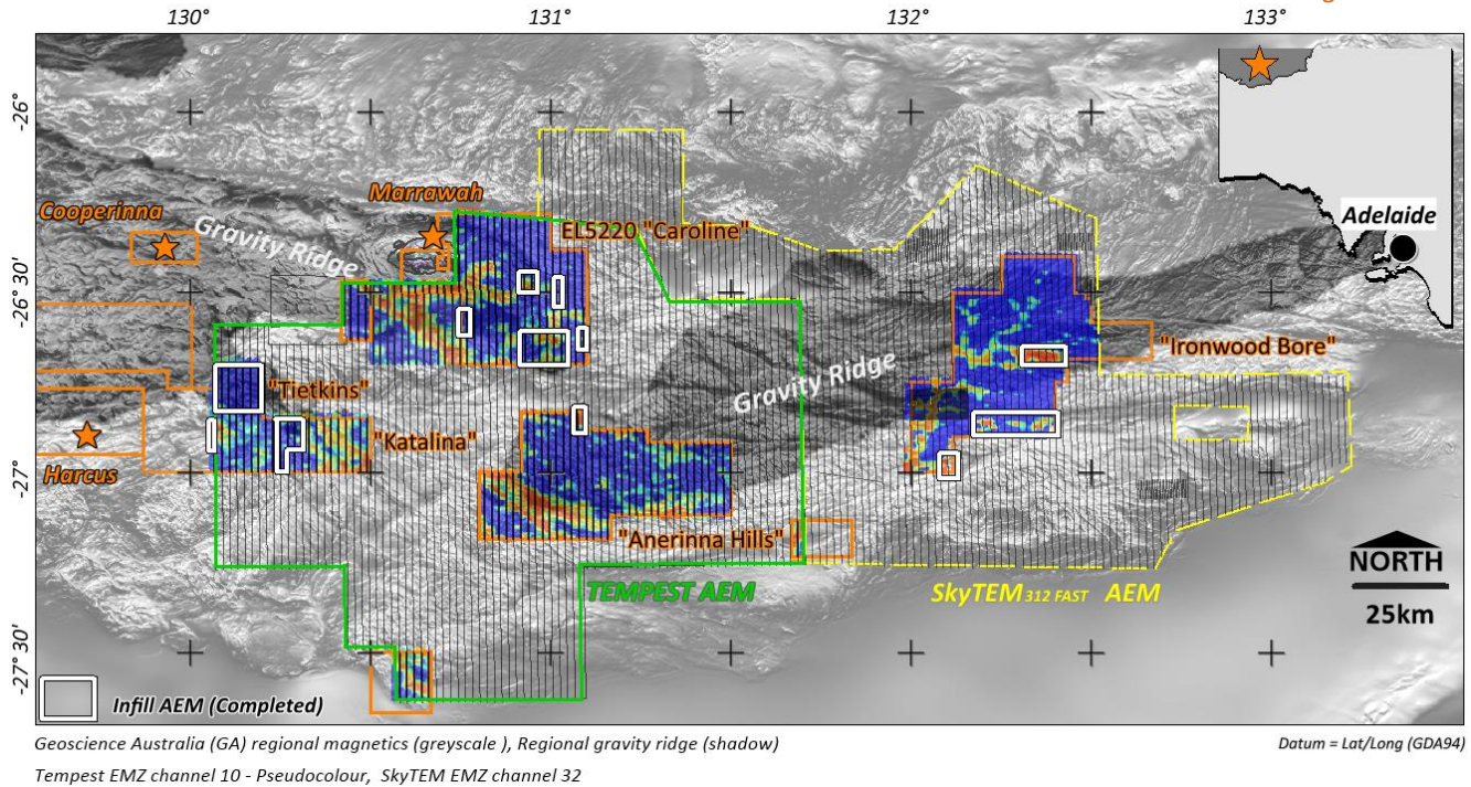
Figure 9: Airborne Electromagnetic Survey Areas - central Musgrave Region South Australia
