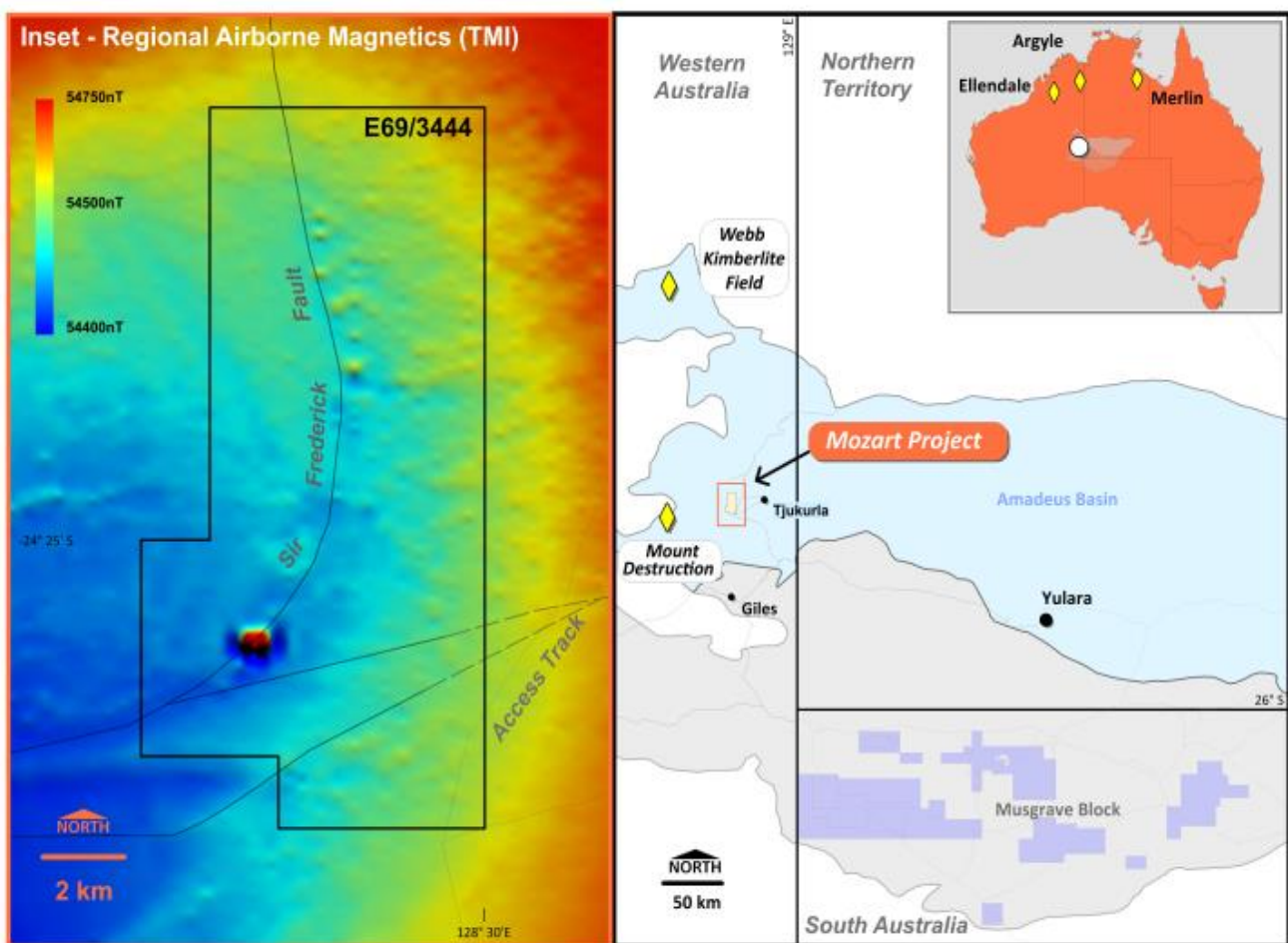
Figure 10 : Mozart Diamond Project - West Amadeus Basin (Western Australia)
