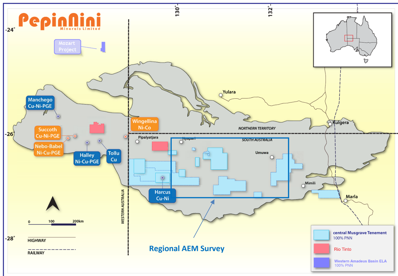
Figure 8 NiCuL Minerals Musgrave Project, South Australia and Western Australia
