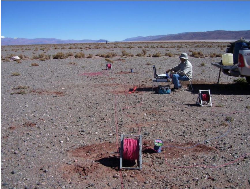
Figure 5 VES Geophysical Survey - Salta Province
