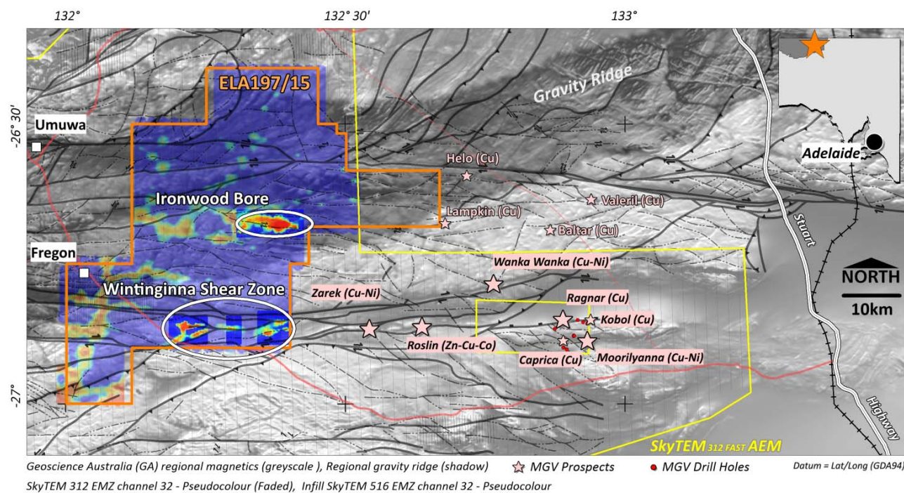
Figure 9: Ironwood Bore AEM anomalies
