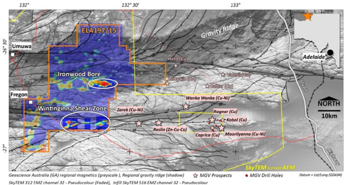
Figure 18 – Ironwood Bore AEM anomalies
