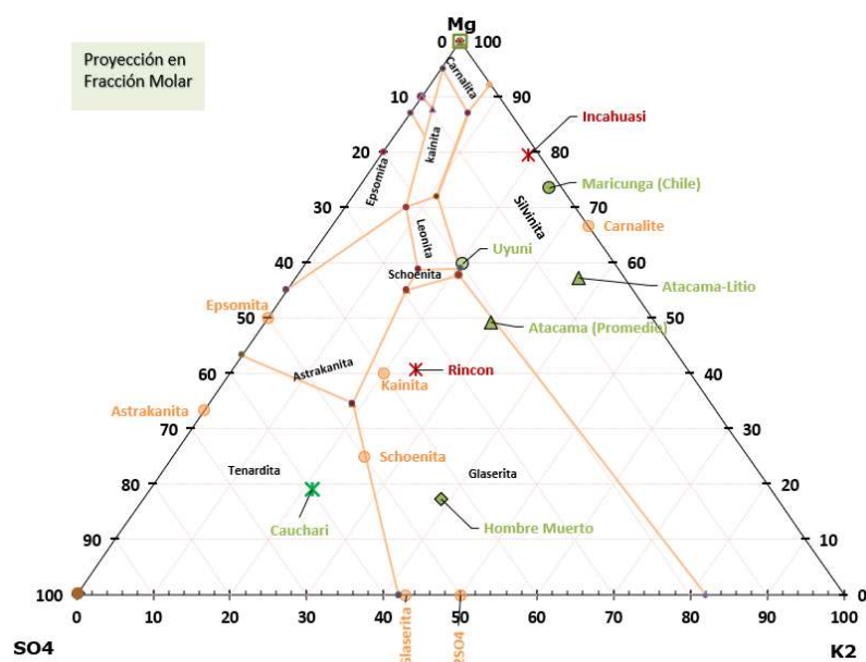
Figure 4 – Phase chemistry for salar comparison
