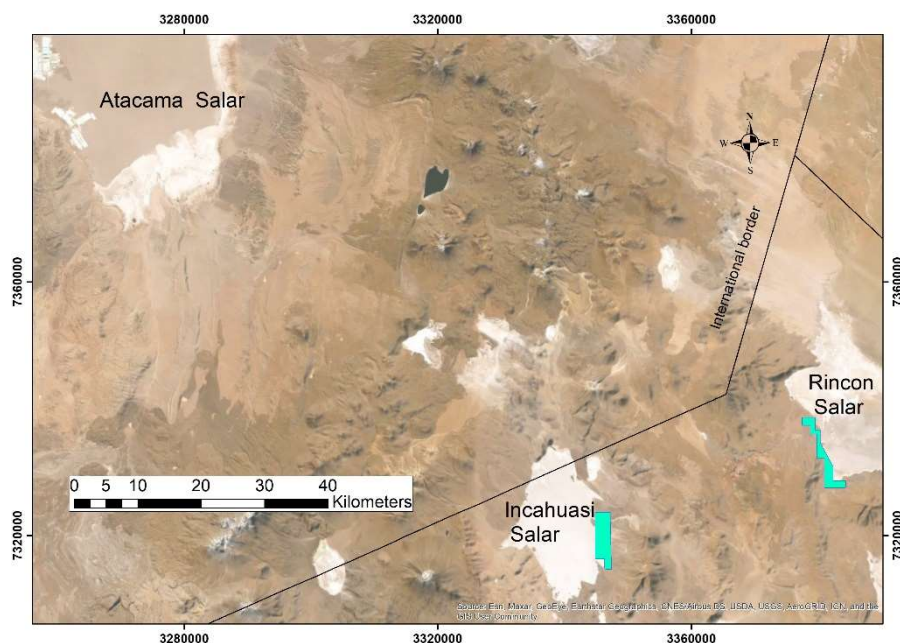
Figure 2 – PNN project locations(Argentina) and Atacama Salar(Chile)
