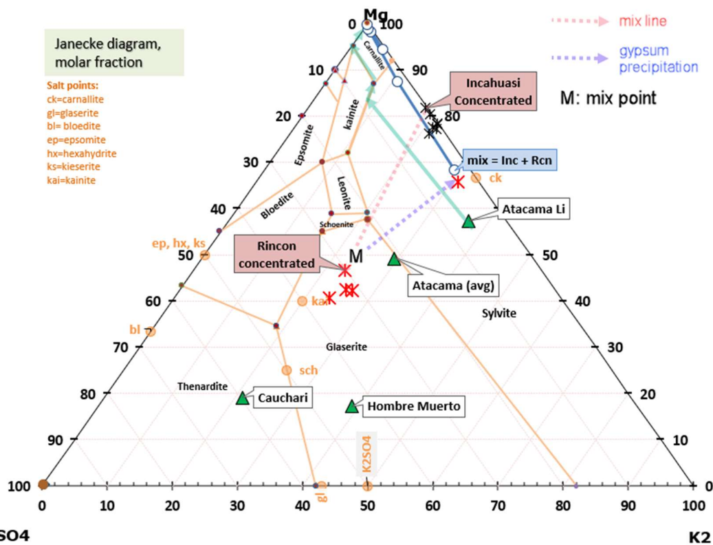
Figure 3 – Phase diagram indicating chemical pathway of the evaporation process
