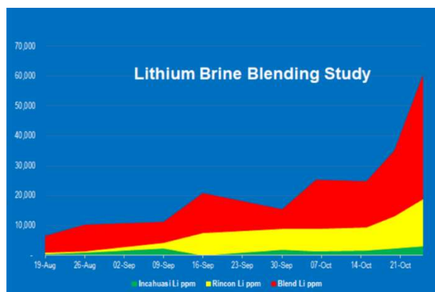
Figure 1 - Lithium ion concentrations against time for mix and individual brines through the evaporation process.
