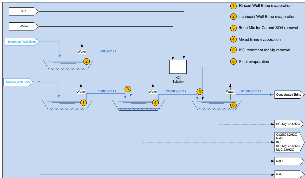
Figure 2: Brine-Blending Evaporation Process Flowsheet, December 2021
