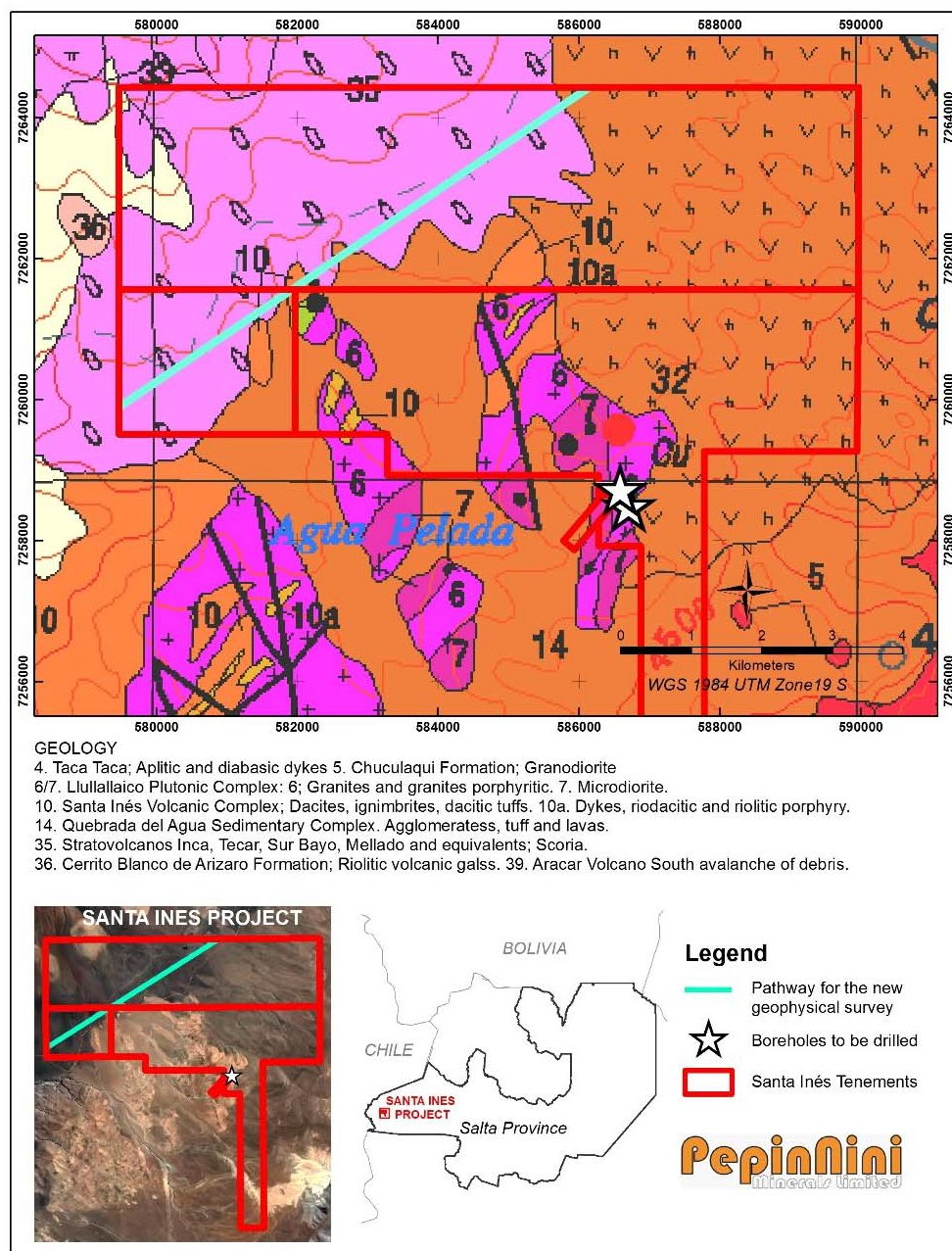
Figure 5: PepinNini-Ganfeng Lithium geophysical survey pathway through the Santa Ines Project
