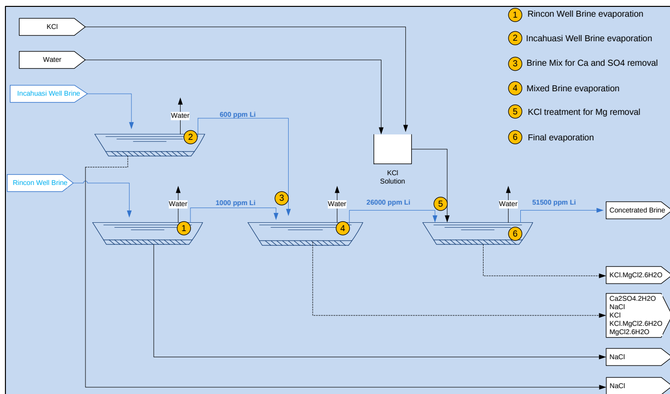
Figure 1: Brine-Blending Evaporation Process Flowsheet
