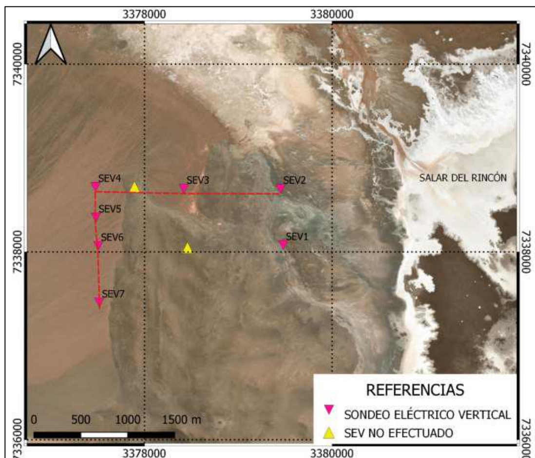
Figure 5: Location of VES geophysics stations (SEV1-7 purple triangles), Rincon North.
