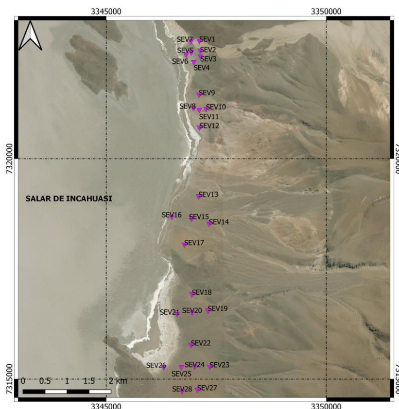
Figure 4: Locations of VES geophysics stations (#1-28 purple dots), Incahuasi salar
