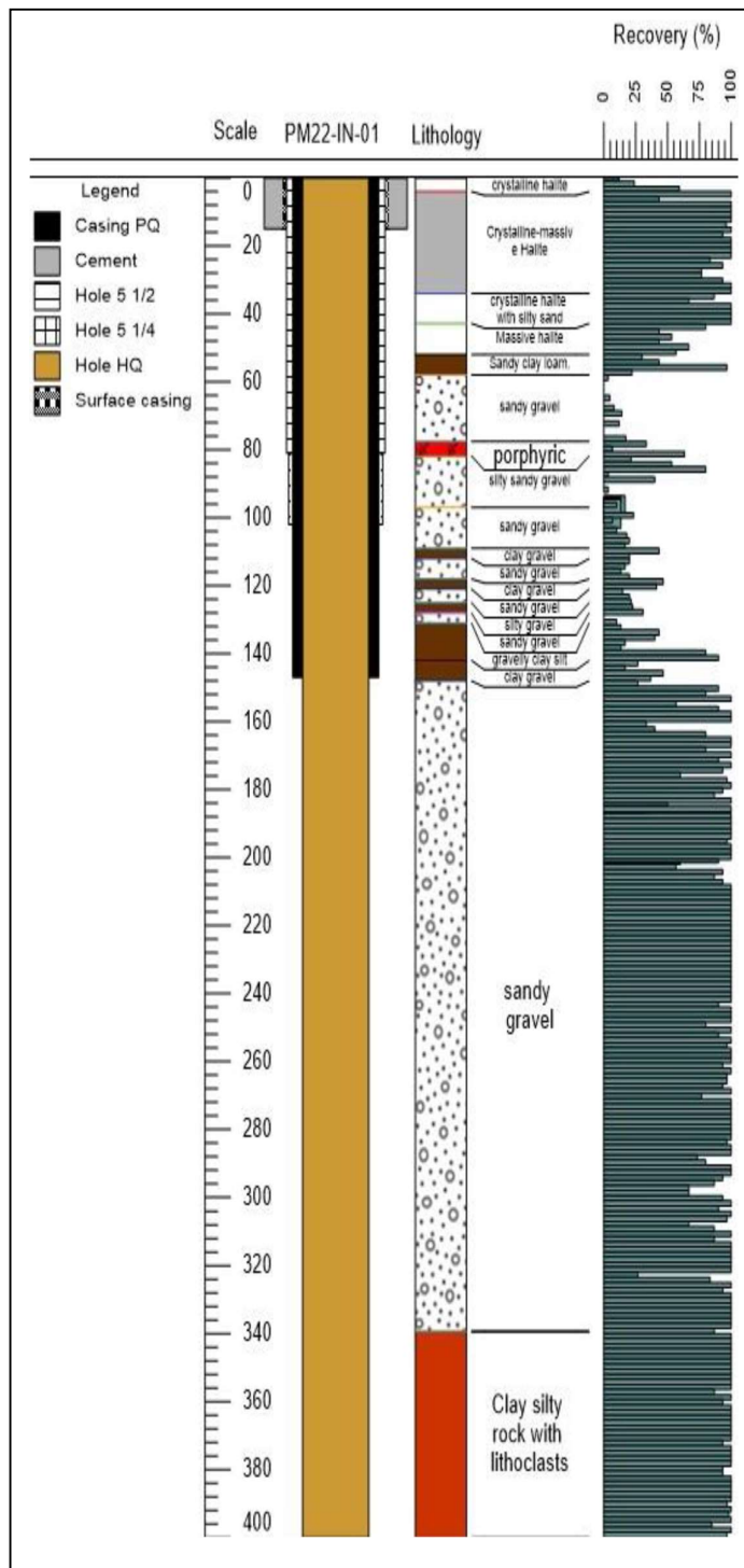
Figure 2a: Summary Drill Hole Log PM22-IN-01
