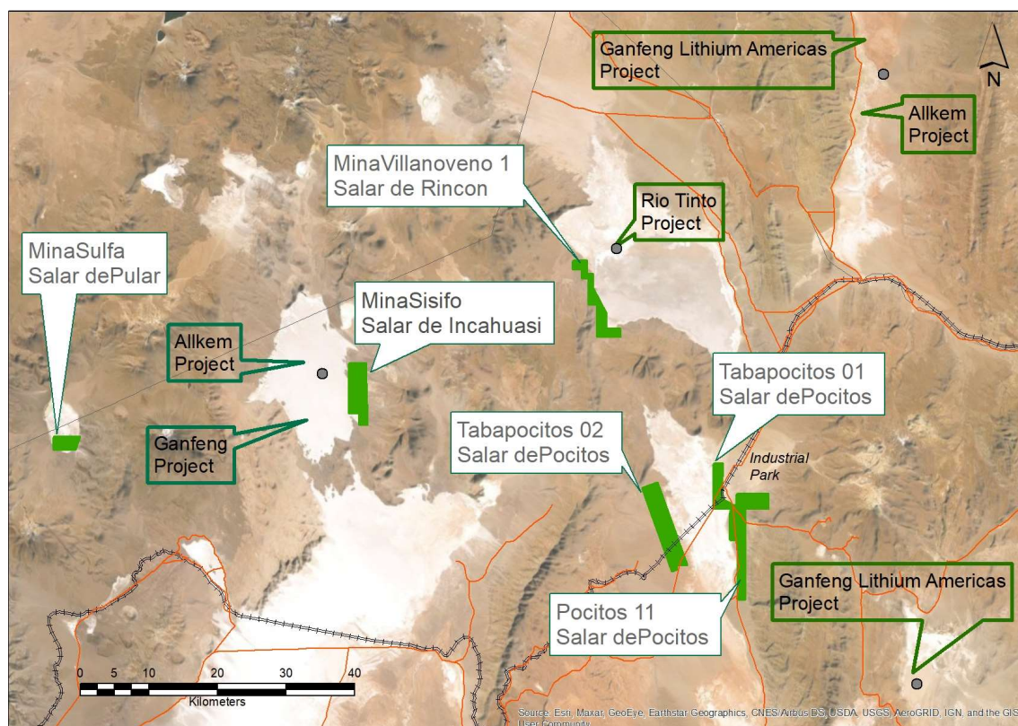
Figure 4: Salta Lithium Brine Project location map, north-west Argentina (PNN licenses in green)
