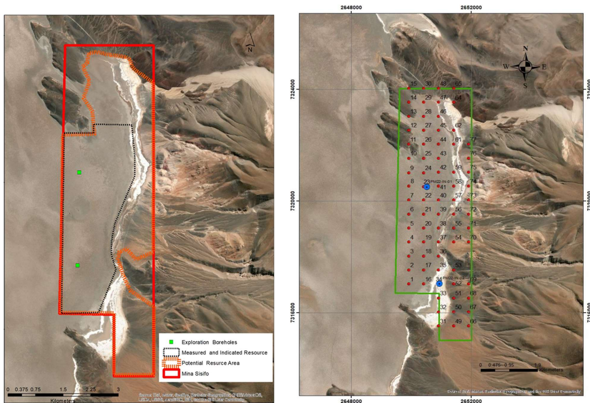
Figure 3a: Incahuasi salar showing location of two planned drillholes (green dots) and potential Resource area Figure 3b: Revised drill hole locations (blue dots) and previous TEM geophysical survey points (red dots)
