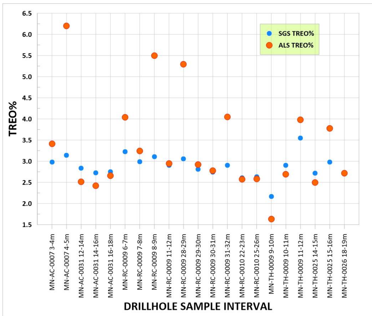
Figure 1: Incomplete original REE assay shown on blue, new complete REE assays shown in orange
